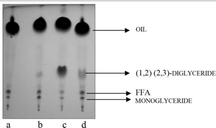
Figure 2. Thin layer chromatogram showing breaking of oil with increasing concentration of oil (lane a – fresh oil [control]; lane b – 8 %; lane c – 16 %; lane d – 18 %) as carbon source during growth of the organisms after 10 day exposure.
