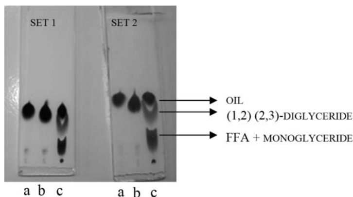
Figure 1. Thin layer chromatogram (in duplicate) showing breaking of oil (lane c) in comparison to pure oil (lane a) and abiotic growth medium with pure oil (lane b) maintained in the same conditions as that of experimental flasks.
