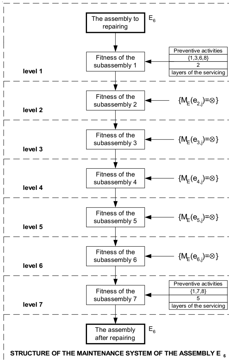
Figure 13. The scheme of structure of the maintenance system of an assembly E_6 .
