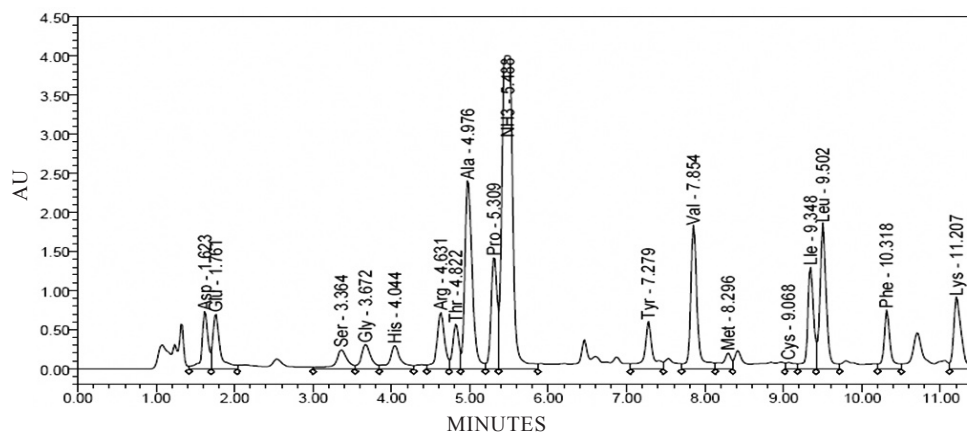
Figure 5. HPLC chromatogram of Allium auriculatum .
