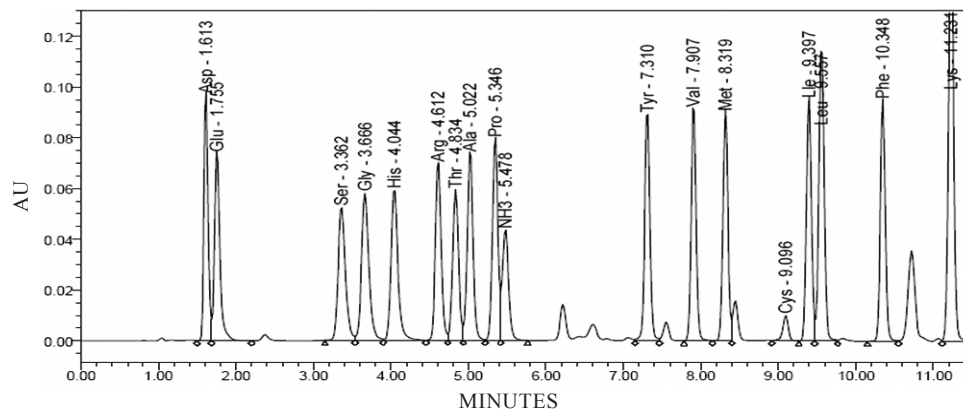
Figure 4. HPLC chromatogram of standard amino acids.
