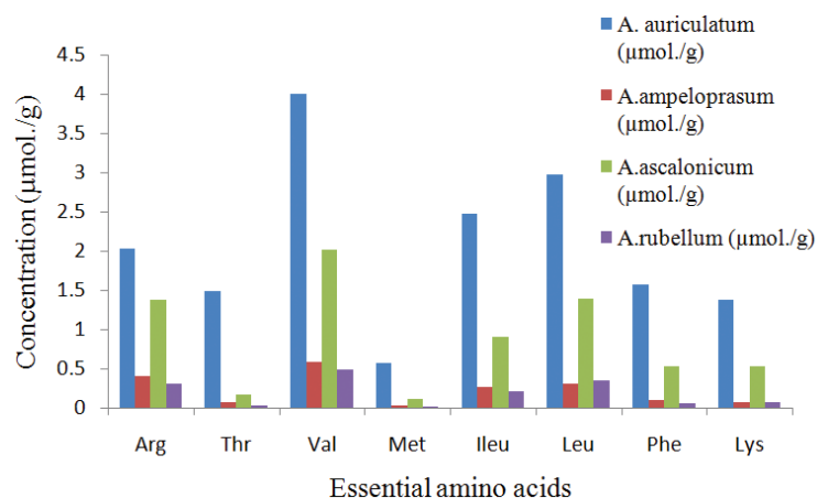
Figure 1. Essential amino acids present in the different Allium species.
