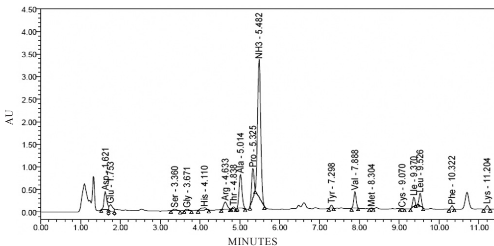
Figure 6. HPLC chromatogram of Allium ampeloprasum .
