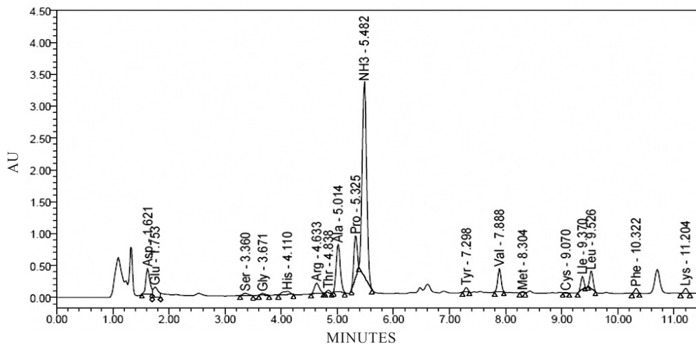
Figure 8. HPLC chromatogram of Allium rubellum .
