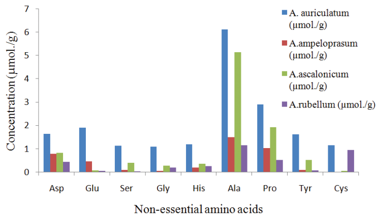
Figure 2. Non-essential amino acids present in the different Allium species.
