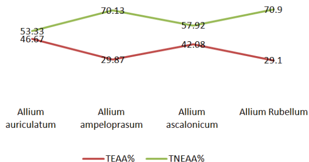
Figure 3. Total essential and non-essential amino acids present in the different Allium species.
