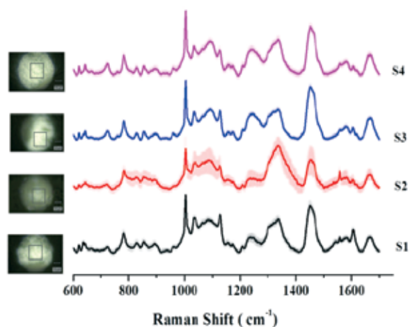
Figure 1: Averaged Raman spectroscopic signal from four strains of Escherichia coli . (S1-S4), where S1 is E.coli ATCC 10536, S2 is E. coli MTCC1687, S3 is E. coli O157:H7 DFRL 302 & S4 is E. coli O157:H7 DFRL 303. The left panel depicts the white light image of the spot from where Raman spectra were acquired.
