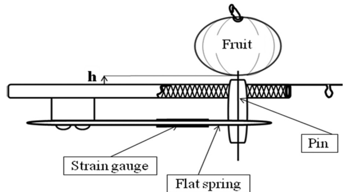
Figure 1. A typical mechanical thumb equipment.
