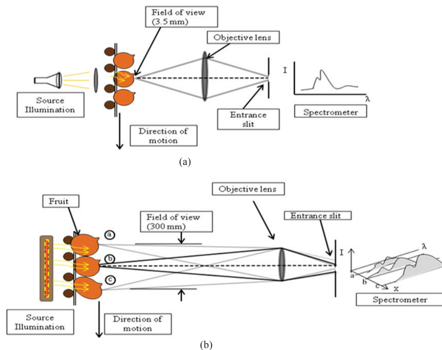
Figure 3. Sequential points in a continuous NIR system: (a) Typical mono and (b) Multiple.
