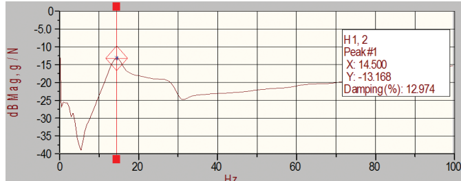
Figure 4. A typical acoustic spectrum with the help of acoustic impulse instrument.
