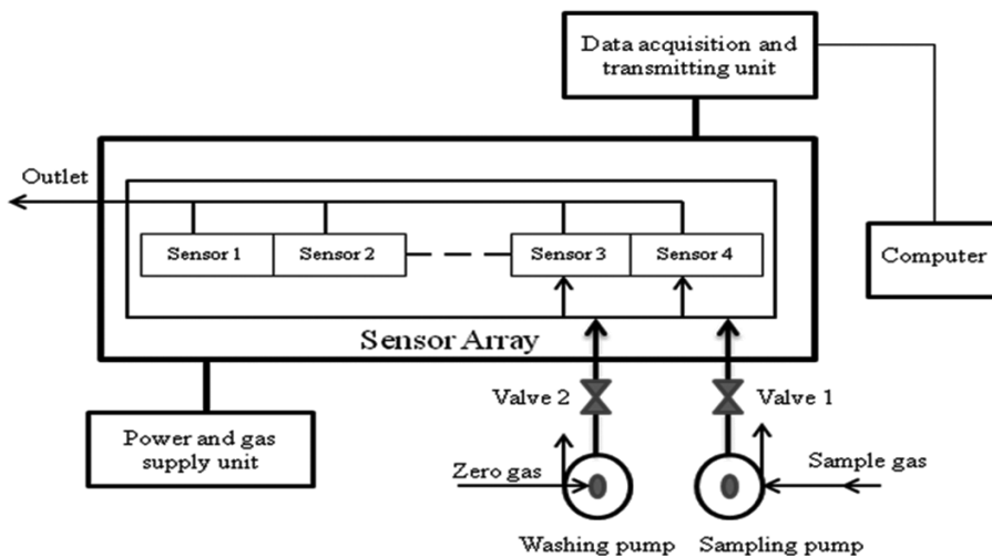
Figure 2. Schematic diagram of an E-nose system.
