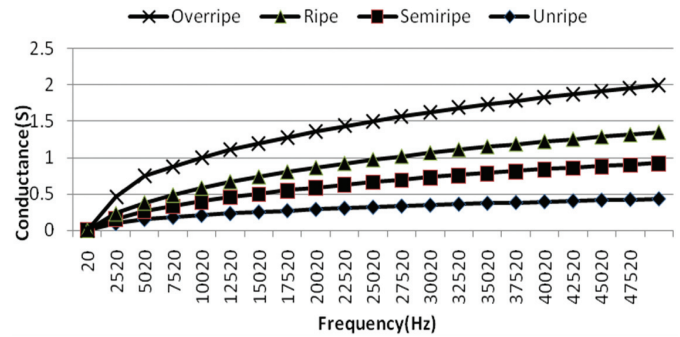
Figure 5. Electrical conductivity of banana at different ripening stages with the help of electrical conductivity monitoring equipment.
