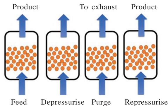
Figure 2. Schematic of the PSA technology showing the cyclic repetition of four basic steps.
