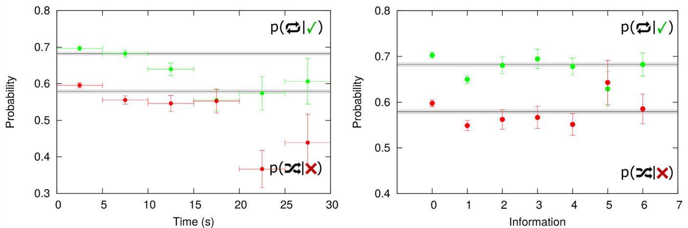
Fig 4. Decision conditioned to performance: the Win-Stay Lose-Shift emerging strategy. Empirical conditional probabilities of repeating previous guess are positively correlated with success and failure of the previous guess. The highest probability corresponds to repeating the previous guess when this was correct (0.682). The expert’s advice partially neutralizes the effect (0.610). (down left) The conditional probability decreases when participants spend more time to make the decision in both cases: being “correct” (green) and being “wrong” (red) in the previous round. (down right) The conditional probability initially diminishes but when a participant consults more information it oscillates around the mean in both cases: being “correct” (green) and being “wrong” (red) in the previous round. Horizontal lines in bottom plots provide aggregated results and shadows their error bars. Error bars represent the Standard Deviation of a binomial distribution.
