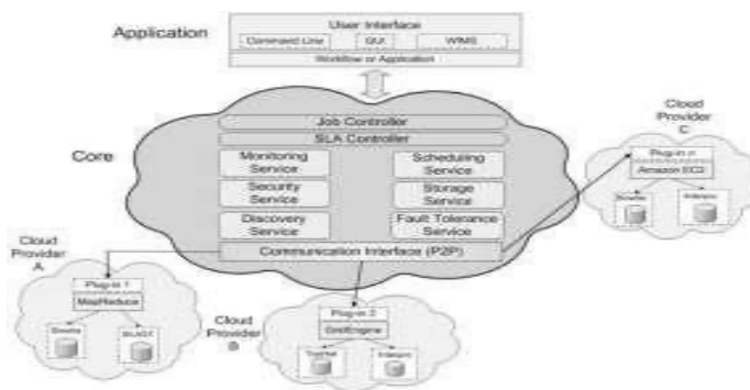
Fig 1. Cloud Architecture
