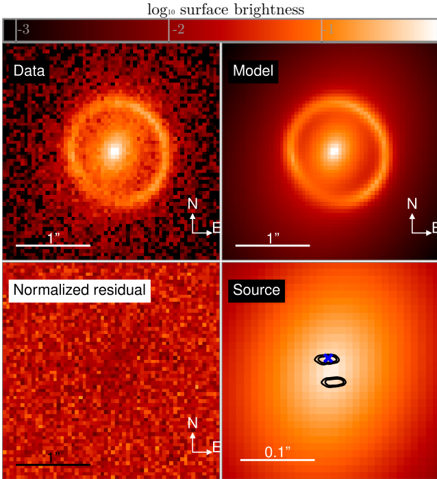
Figure 4. The sample lens system we use in our simulated Hubble constant measurement. Top-left panel: Observed light distribution. Top-right panel: Best fit model of the lens and the source. Bottom-left panel: The difference after subtracting the model from the data. Bottom-right panel: The reconstruction of the non-lensed source for the best fitting model, and the inferred position of the binary black hole relative to the source at 68% and 90% confidence (black contour) as well as its true position (blue cross). Our final sky localization is factor \sim 10^9 times better than the initial localization by LIGO/Virgo/Kagra ( \sim 4 \text{ deg}^2 ).
