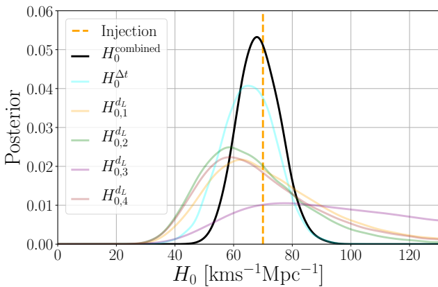
Figure 5. Measurement of the Hubble constant H_0 from the combination of gravitational-wave data and the lensed EM host galaxy (black). The coloured lines show the H_0 inferred from each of the four lensed gravitational wave ‘standard siren’ posteriors and the time-delay distance measurement (cyan). Combining these constraints yields a more stringent H_0 measurement compared to the individual posteriors. The dashed line shows the simulated value of H_0 = 70 \text{ kms}^{-1} \text{ Mpc}^{-1} .
