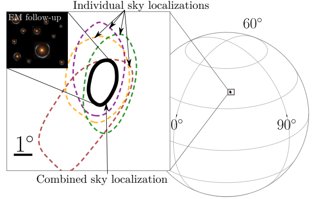
Figure 1. An illustration of a sky localization of a quadruply lensed gravitational wave. We show both the individual (color) and the combined (black) sky localizations at 90% confidence. Each lensed gravitational-wave essentially gives us a new set of detectors with which to localize the event in the sky, allowing for improved sky localization. A dedicated follow-up of the narrowed sky region would then allow us to search for the lensed host galaxy from which the gravitational-wave originates.
