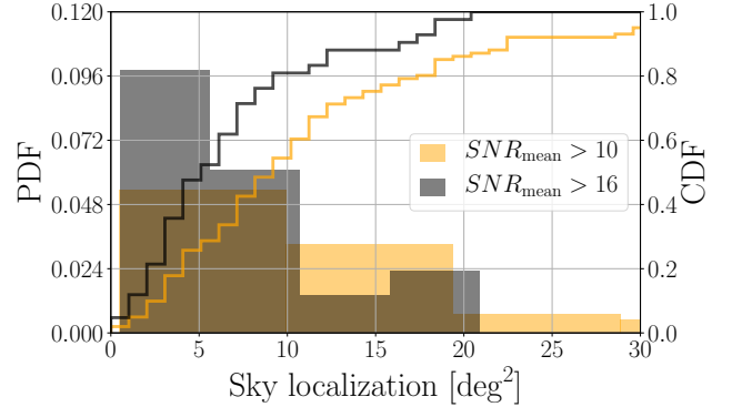
Figure 2. The probability (histogram) and cumulative distribution function (lines) of the combined sky localization constraints for our catalog of quadruply lensed events in the low (orange) and moderate (black) mean signal-to-noise ratio regimes. We have combined the sky localization posteriors of the four individual lensed events. At both low and moderate signal-to-noise ratio, a large fraction of the events are constrained to better than 10 \text{ deg}^2 in the sky, and often to better than 5 \text{ deg}^2 . We quote the 90% confidence interval for the sky localization.
