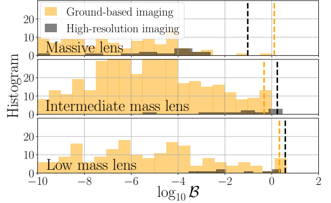
Figure 3. The Bayes factor in favor of a given galaxy being the host of the merging black hole. We show the results for 550 lens reconstructions within the sky localization of the injected gravitational-wave using ground-based imaging (orange). The Bayes factor for the 11 best fitting lenses are shown in black after modeling simulated high-resolution follow-up imaging. The Bayes factors are large for lenses that can reproduce the observed lensed GW event properties, and low for lenses that are inconsistent with producing the observations. We show three lensing configurations: a gravitational-wave lensed by a massive \sim 2 arcsec Einstein radius lens (top panel), a moderate \sim 1 arcsec lens (middle panel), and a small \sim 0.5 arcsec lens (bottom panel). The correct lens yields a high Bayes factor in all three cases (vertical dashed lines). In the massive lens scenario (top panel), the background of lensed galaxy candidates is separated. Thus, we can uniquely narrow down the source to one galaxy at above 90% confidence with high-resolution imaging. In the moderate and small lens scenarios (middle and bottom panels), we narrow down the host galaxy to four and five candidates, respectively.
