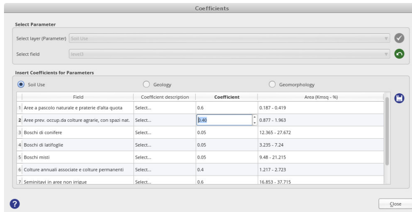
Figure 3. Graphical User Interface of stage 2. The user can select a preloaded coefficient value from Coefficient description column or insert manually a value in the Coefficient column.
