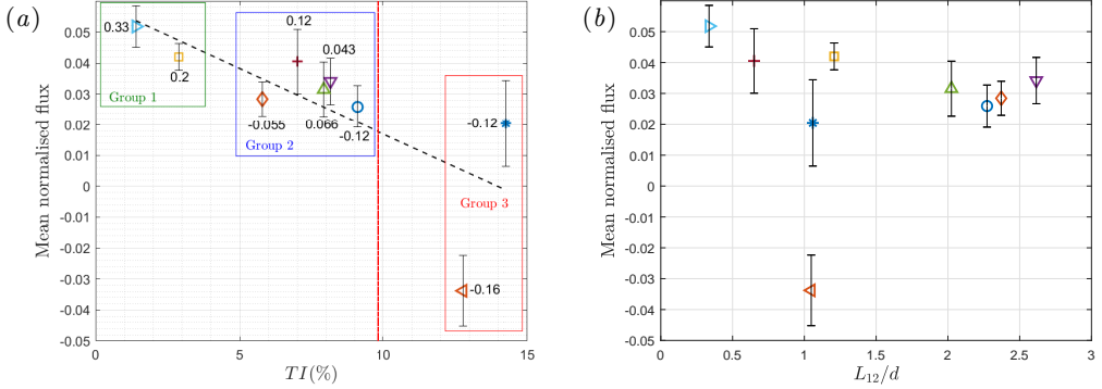
FIGURE 14. Entrainment mass flux as a function of (a) subjected free-stream turbulence intensity and (b) length scale (positive value indicates entrainment into the wake from the background). The dashed line indicates a linear regression fit. Text next to each datapoint indicates the skewness of the respective dataset. The error bars represent a 95% confidence interval. The red dot-dashed line indicates the turbulence intensity near the centerline of the baseline (no-grid) wake.
