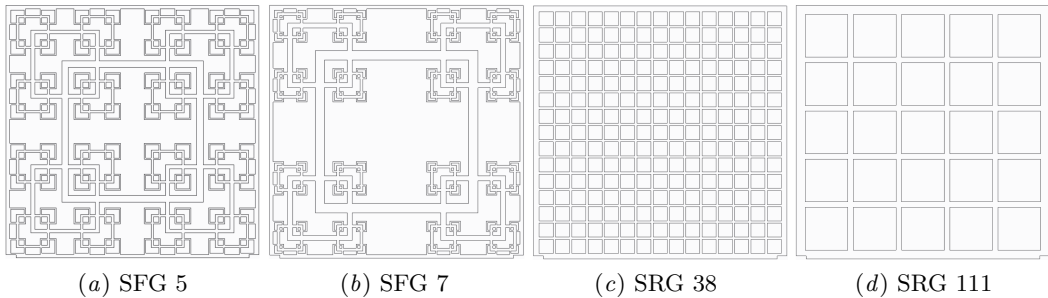
FIGURE 1. Schematic of turbulence generating grids: (a) & (b) display the fractal square grids, whereas, (c) & (d) depict square regular grids.
