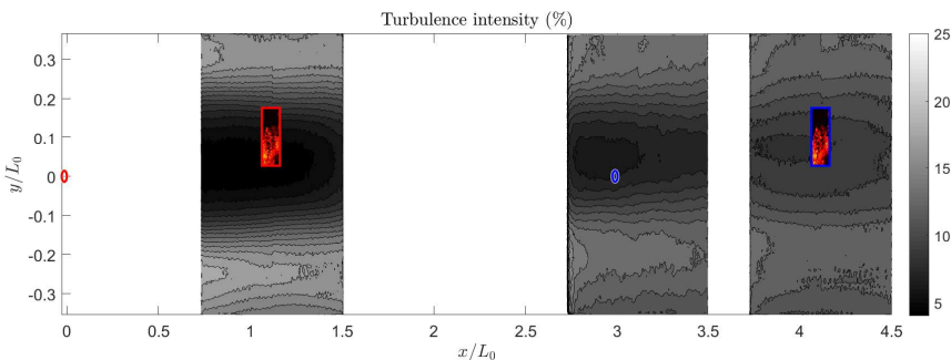
FIGURE 22. Turbulence intensity profile downstream of a square regular grid with \mathcal{L}_0 = 354 mm. The overlays represent the investigated FOVs. The positioning of the grid, cylinder and the experimental FOV is consistent with that of run 2a for the red outline. Whereas the blue outline highlights the positioning for run 2e.
