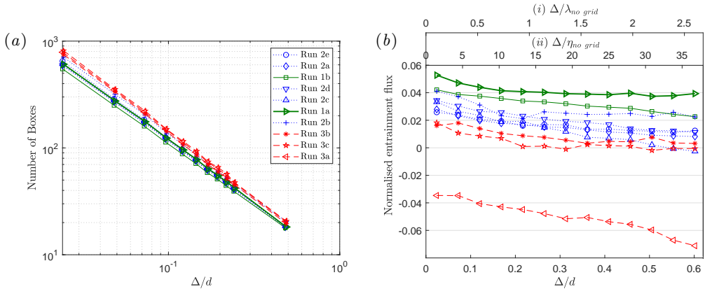
FIGURE 17. Multi-scale analysis. (a) Number of boxes covered by the wake boundary as a function of the box size used. (b) Scale by scale normalised entrainment flux. Note, the two axes on the top of the plot represent the filter size normalised by (i) Taylor length scale ( \lambda ) and (ii) Kolmogorov length scale ( \eta ) found inside the wake, when calculated for the no-grid case.
