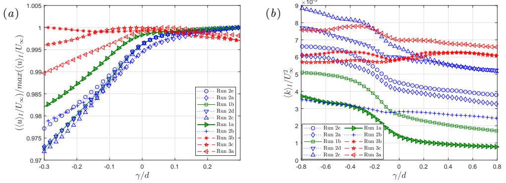
FIGURE 8. Interface conditioned statistics as a function of normal distance away from the wake boundary. (a) Normalised mean velocity. u and U_\infty refer to the stream-wise velocity and the stream-wise mean velocity respectively; (b) Turbulent kinetic energy, k , normalised by U_\infty^2 .
