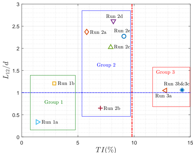
FIGURE 6. Free-stream turbulence parameter envelope. Note that the red dot-dashed line indicates the turbulence intensity near the centerline of the wake in the no-grid case, whereas the dotted blue line indicates a length scale equal to 1 cylinder diameter.
