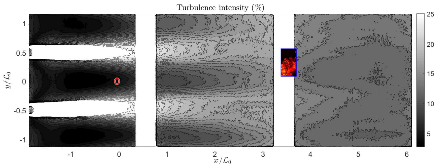
FIGURE 16. Turbulence intensity profile downstream of a square regular grid with \mathcal{L}_0 = 111 mm. The overlay represents the investigated FOV. The positioning of the grid, cylinder and the experimental FOV is consistent with that of runs 3b & 3c. Note that similar figures depicting the flow downstream of all grids used in this study can be found in appendix A.
