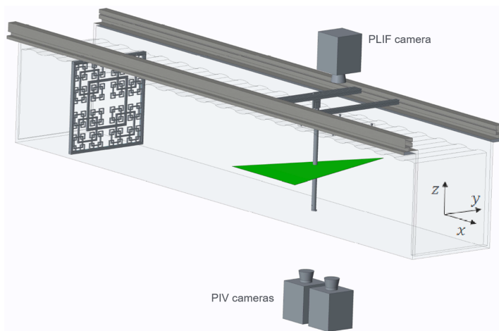
FIGURE 2. An example of the experimental setup used for a typical run. The laboratory coordinate system is also shown. Note that for clarity, the coordinate system has not been plotted on the origin (which lies on the rear face of the circular cylinder), instead it has been shifted downstream in the stream-wise direction.
