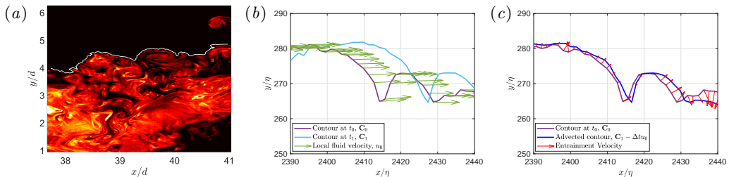
FIGURE 13. (a) A typical PLIF image. The solid white line represents the interface as identified by the gradient metric. (b) & (c) Plots depict the entrainment velocity calculation process. Note that \eta represents the Kolmogorov length scale.
