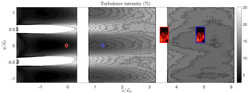
FIGURE 19. Turbulence intensity profile downstream of a square regular grid with \mathcal{L}_0 = 111 mm. The overlays represent the investigated FOVs. The positioning of the grid, cylinder and the experimental FOV is consistent with that of runs 3b & 3c for the red outline. Whereas the blue outline highlights the positioning for run 3a.
