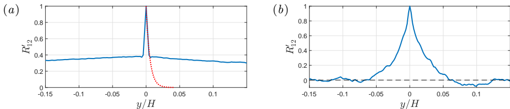
FIGURE 5. Transverse correlation function for stream-wise fluctuating velocity. (a) Correlation function in an empty tunnel. Note that the dashed red line represents the exponential fitted to the short range correlation peak. (b) Typical function downstream of a turbulence generating grid. Note, H represents the width of the flume’s working section.
