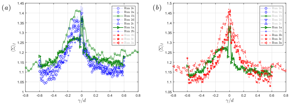
FIGURE 9. Interface anisotropy for turbulence cases in (a) groups 1 and 2; (b) group 3.
