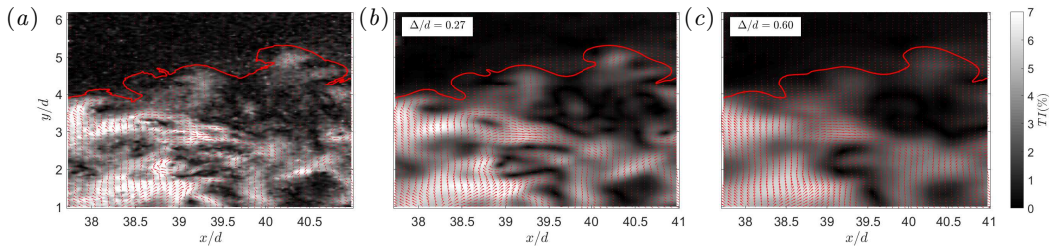
FIGURE 18. Illustration of the filtering process conducted for the multi-scale analysis. Plots depict the turbulence intensity field superimposed by velocity vectors and the wake boundary for the no-grid case. Note that only one in three velocity vectors are displayed for clarity. (a) Unfiltered (b) Filter size, \Delta/d = 0.27 (c) Filter size, \Delta/d = 0.60
