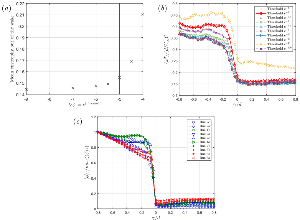
FIGURE 3. Threshold sensitivity study. Note, (a) and (b) refer to the no-grid case. (a) Plot showing the mean normalised entrrophy considered to be outside of the wake for varying gradient threshold values. (b) The variation of interface conditioned entrrophy jump for various threshold values. The thick red line represents the chosen threshold. Note that the boundary contour is different for each threshold value as the location of the contour is dependent on the threshold. (c) Interface conditioned plot of PLIF light intensity normalised by the maximum value for -0.8 < \gamma < 0.8 , calculated using the chosen threshold value.
