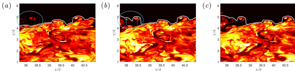
FIGURE 24. Artificial cliffs in the contour as a result of eddies entering the field of view. (a) Snapshot at time, t_0 (b) Snapshot at time, t_0 + \Delta t (c) Snapshot at time, t_0 + 2\Delta t
