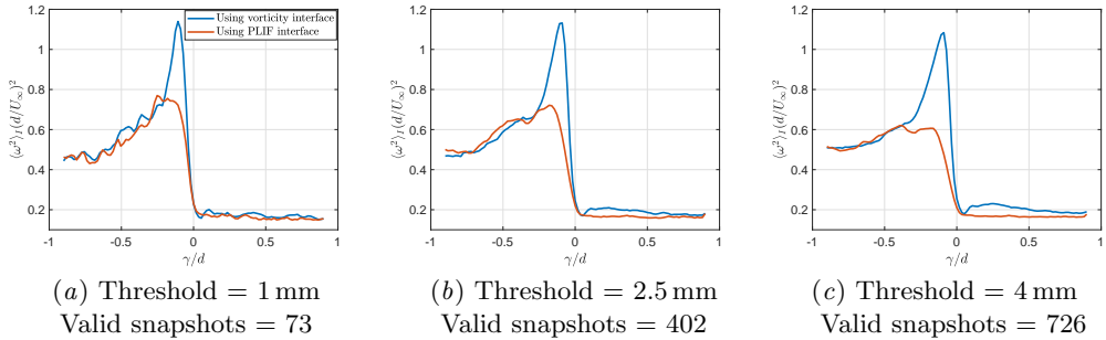
FIGURE 23. Interface conditioned statistics as a function of normal distance away from the wake boundary identified by both the PLIF data as well as the vorticity data. The series of figures illustrate the sensitivity to the chosen threshold. Captions of each subfigure represent the chosen threshold difference between the contours identified using the two different methodologies as well as the number of valid snapshots that consist of valid contours using both methodologies and pass the threshold test.
