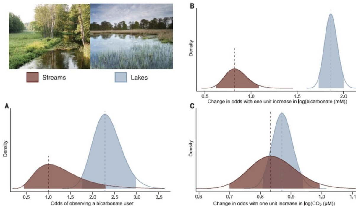
Fig. 1. Bicarbonate use in submerged freshwater plant communities. (A) Likelihood of observing a bicarbonate user versus a CO 2 user in streams ( n = 172 samples; red) and lakes ( n = 791 samples; blue). (B and C) Modeled odds of observing a bicarbonate user versus a CO 2 user as a function of bicarbonate (B) or CO 2 (C)
