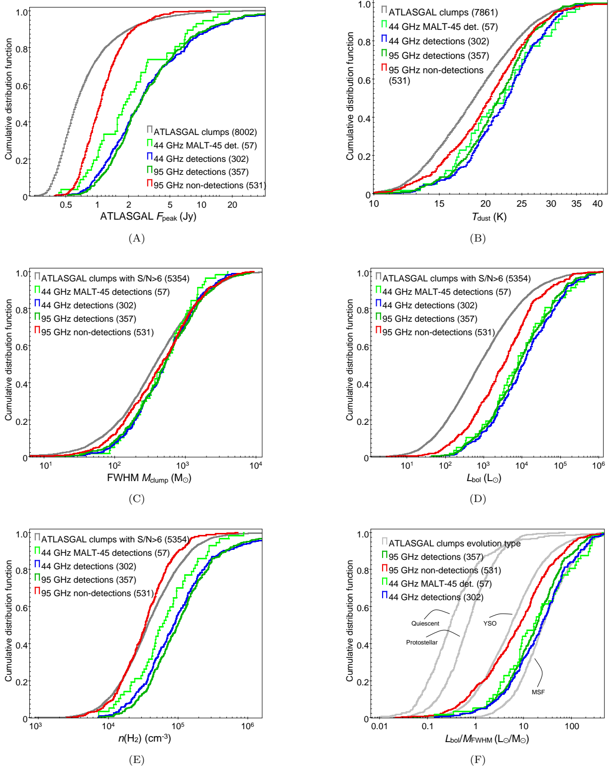
Figure 4. Cumulative distribution plots of clump physical parameters ((A) peak flux density, (B) dust temperature, (C) FWHM mass, (D) bolometric luminosity, (E) number density and (F) luminosity to clump mass ratio) associated with class I methanol masers. The gray line shows all ATLASGAL sources ( 280^\circ < l < 60^\circ , |b| < 1.5^\circ ) with defined parameters. The green and red lines show those ATLASGAL clumps with an observed detection and non-detection of 95 GHz masers, respectively. The blue line is maser-associated clumps at 44 GHz. The light green line shows the sources with 44 GHz masers detected in the MALT-45 survey (Jordan et al. 2015; 330 < l < 335 , |b| < 0.5^\circ ). In the last panel (F) grey lines show the different evolution types of all ATLASGAL sources, marked with labels.
