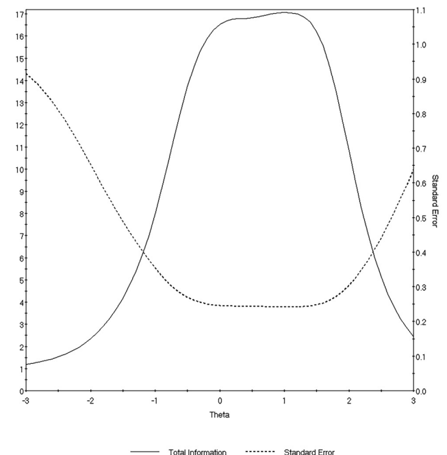
Fig. 4. Test information curve
