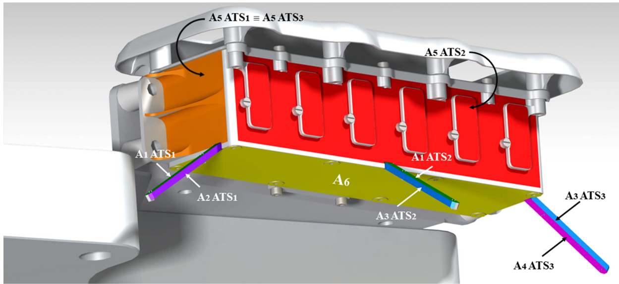
Fig. 10. Radiating surfaces considered for the heat exchange at the thermal radiation model. The view factors have been estimated by simplifying the geometry of the real surfaces A_1 to A_6 to rectangles of the same dimensions and area. The disposition and the value of the surfaces A_1 to A_4 are similar for each ATS rod, surface A_6 is also common to all the ATS rods, and surface A_5 is different for ATS rod 2 (red surface) with respect to the other two sensors (orange surface). For interpretation of the references to colour in this figure legend, the reader is referred to the web version of this article.
