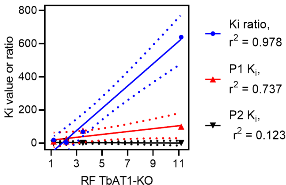
Figure 3: Correlation plot between the Resistance Factor (RF) of compounds 5 , 6 , 7 , 12 , and 22 and their K_i for the P1 transporter (red line and symbols), the K_i for the P2 transporter (black line and symbols), and their ratio (P1/P2; blue line and symbols). 95% confidence intervals are indicated by dotted lines and correlation coefficient r^2 is given for each line.
