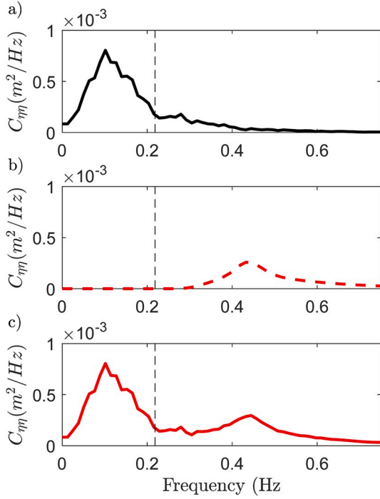
Fig. 3. Example of a) the IG-wave spectrum based on the computed surface elevation; b) an assumed SS-wave spectrum (JONSWAP shape) based on the computed root-mean-square SS-wave height ( H_{rms} ); and c) the total combined spectrum, for XB-SB at the dike toe (steep wind-wave case).
