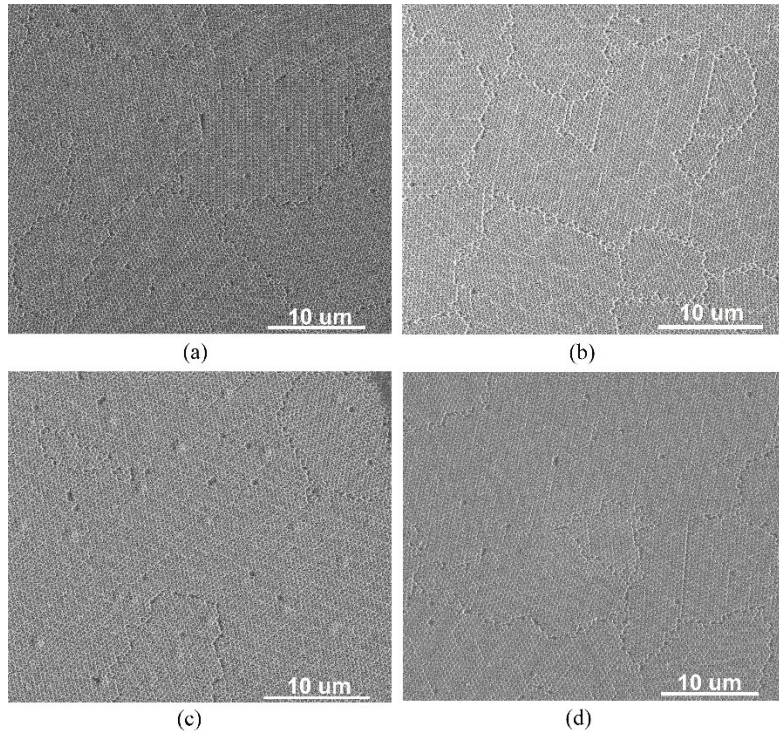
Figure 4. Scanning electron microscopy (SEM) images of the samples labeled with the SAM (a), cleaned with oxygen plasma and then relabeled with the SAM (b) or cleaned with hydrogen plasma with different plasma powers and relabeled with the SAM (c, d).
