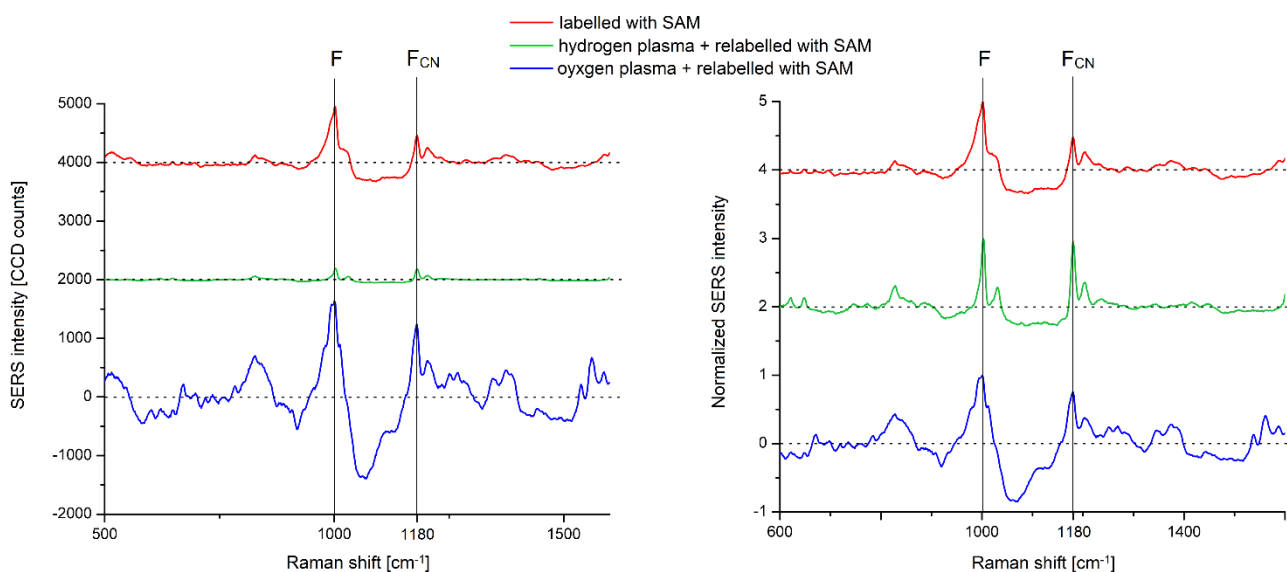
Figure 1. SERS spectra of the samples labeled with the SAM (red), cleaned with hydrogen plasma and then relabeled with the SAM (green) or cleaned with oxygen plasma and relabeled with the SAM (blue). (a) Background-subtracted SERS spectra acquired with identical acquisition conditions. (b) SERS spectra from (a), normalized on their respective highest peak intensities. The dashed horizontal lines represent the zero line of each spectrum, whereas the full vertical lines mark the SERS peaks of the aromatic amino acids.
