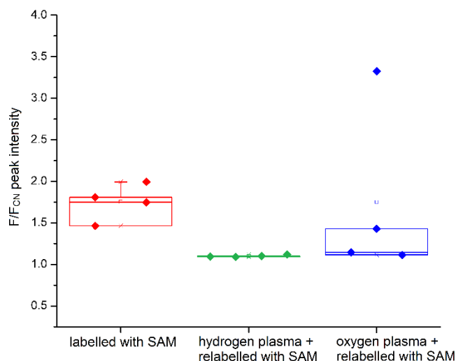
Figure 3. F/F_{\text{CN}} peak intensities for the samples labeled with the SAM (red), cleaned with hydrogen plasma and then relabeled with the SAM (green) or cleaned with oxygen plasma and relabeled with the SAM (blue). The points represent the averaged values on individual samples, whereas the box plot represents the statistical distribution of the points.
