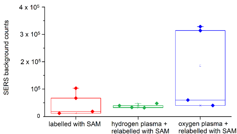
Figure 2. SERS background counts integrated between 500 and 1500 \text{ cm}^{-1} for the samples labeled with the SAM (red), cleaned with hydrogen plasma and then relabeled with the SAM (green) or cleaned with oxygen plasma and relabeled with the SAM (blue). The points represent the averaged values on individual samples, whereas the box plot represents the statistical distribution of the points.
