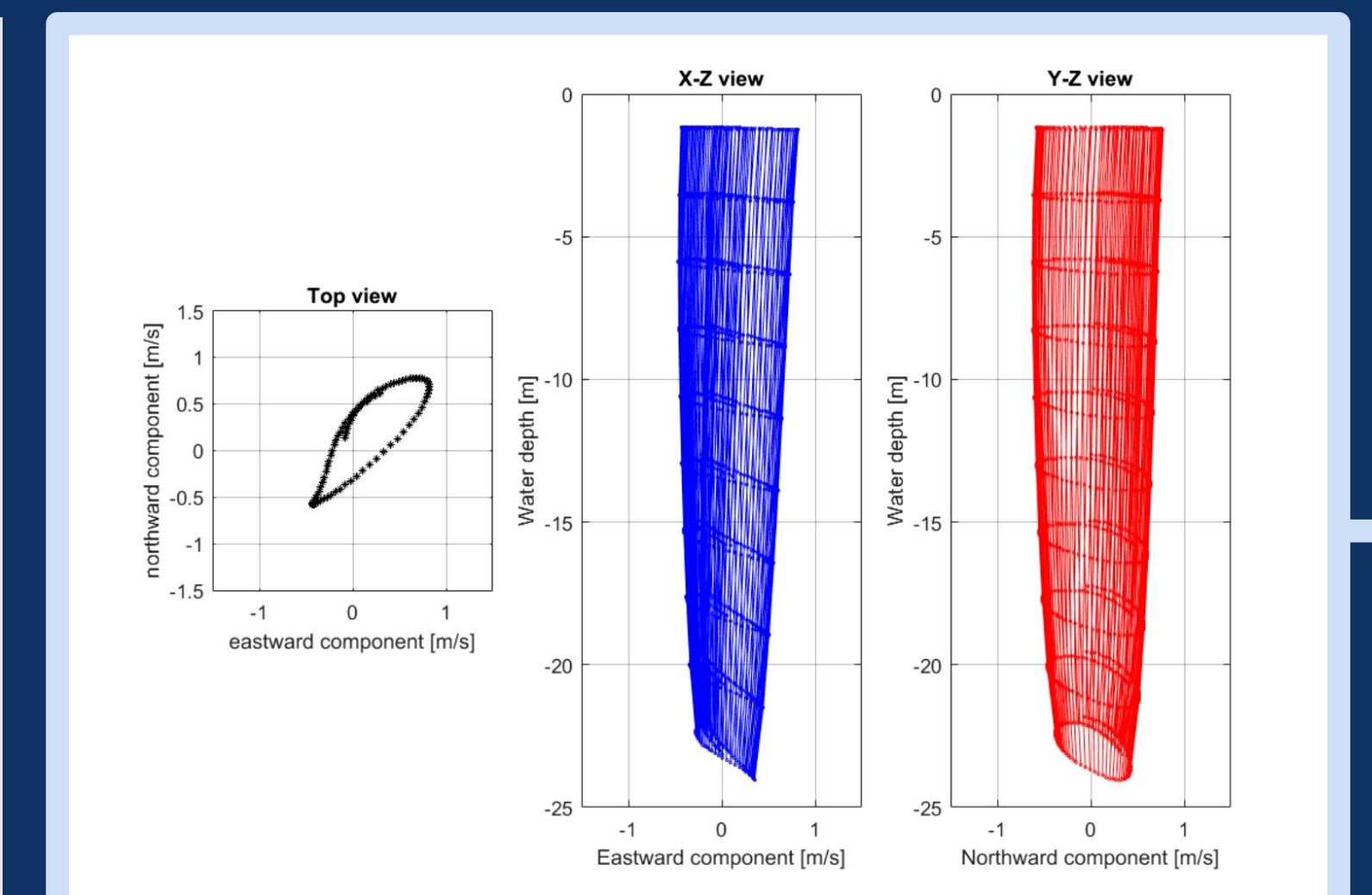
Current velocity profile
