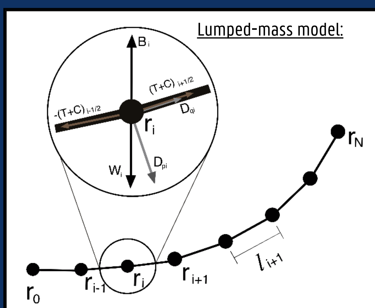
Illustration of a semi submerged longline system that is considered for the study. (length not drawn to scale)
