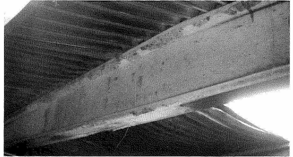
Fig. 3 Fire damage of roof girder
