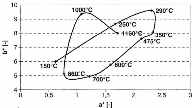
Fig. 1. Colorimetric path of traditional concrete with masked aggregates.
