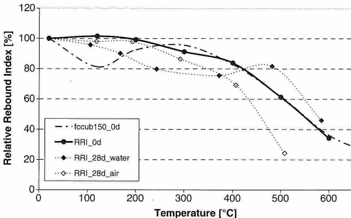
Fig. 2 Decrease of Rebound Index as function of temperature and storage conditions for traditional siliceous concrete
