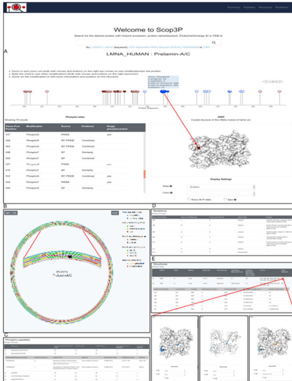
Figure 1. Scop3P web-interface reveals different context information at different levels for all phosphosites in a phosphoprotein.
