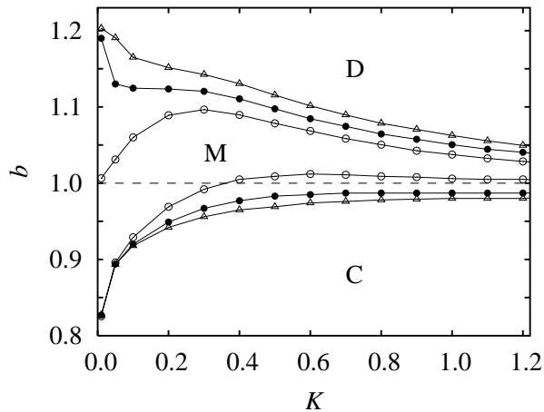
FIG. 4: The lower b_{c1}(K) and upper b_{c2}(K) critical points on the Newman-Watts structure for different p values. The symbols correspond to p = 0.02 (open circle), 0.06 (full circle), and 0.10 (triangle). Solid lines are guide to the eye and dashed line indicates a base line at b = 1 .
