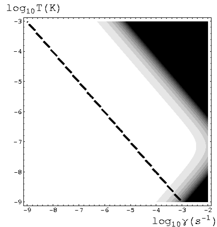
FIG. 1: Contours of equal visibility (white for good, black for poor), as a function of temperature T and friction \gamma ; based on Eqs. (11), (12), (14). Upper-right corner, present-state possibilities; dashed line, where CLS decoherence becomes observable. The turnback of the contours in the lower-right corner corresponds to the coordinate diffusion contribution [8], with \kappa = 1 and \lambda = 1 .
