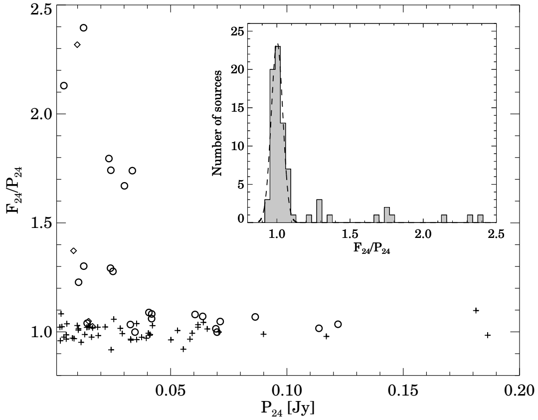
FIG. 2.— Flux ratio of the measured to the predicted flux densities as a function of the predicted photospheric fluxes for our sample stars measured at 24\mu\text{m} with MIPS. For symbols see the caption of Fig. 1. Small panel: the histogram of the flux ratio. The peak at around unity can be fitted by a Gaussian with a mean of 1.00 and dispersion of 0.038 (dashed line). We note that the disks around HD 15745, HD 35841 and HD 221853 with flux ratios of 9.79, 3.39, and 3.87, respectively, are out of the displayed range.
