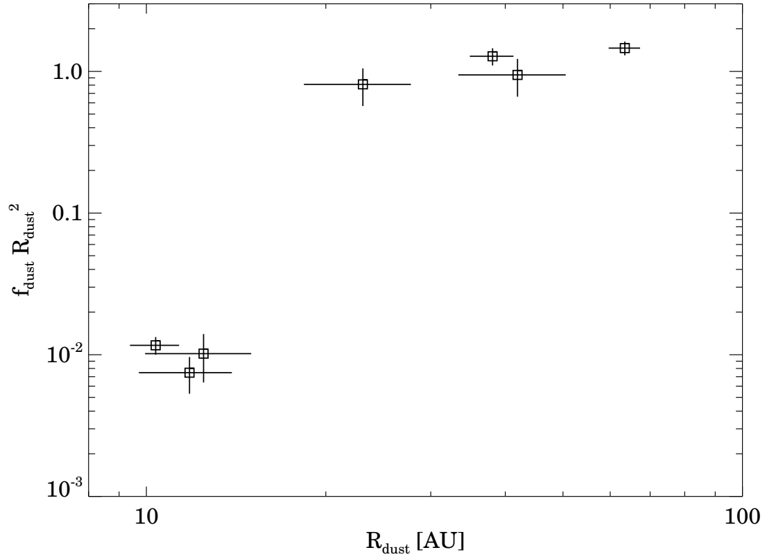
FIG. 17.— The relative dust masses ( f_{\text{dust}} \cdot R_{\text{dust}}^2 see Sect 5.5) for the disks with ages of 30 Myr as a function of the derived radii.
