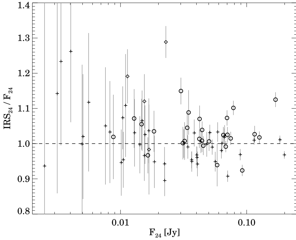
FIG. 5.— The ratio of the synthetic IRS 24μm photometry to the MIPS photometry at 24μm as a function of the MIPS flux densities. For symbols see the caption of Fig. 1. The mean of the IRS_{24}/F_{24} ratios is 1.02 with a dispersion of 0.06. The dashed line corresponds to the IRS_{24}/F_{24} ratio of 1.
