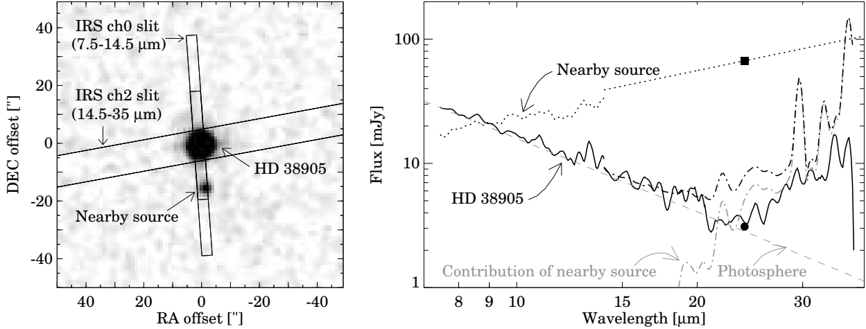
FIG. 6.— Left : 2MASS K_s image of HD 38905 and its surroundings. The position of the two Spitzer/IRS slits are overlaid. A nearby source at a distance of 13.5'' is included in the ch0 slit. At these wavelengths, the two sources are well resolved, and a separate spectrum for each source can be extracted. The ch2 slit is nearly perpendicular to the ch0 slit, but due to the longer wavelength, the PSF is wider, thus the nearby source might have a contribution to the ch2 spectrum extracted for HD 38905. Right : the solid black line indicates the spectrum extracted at the position of HD 38905, and the black dot is a MIPS 24\ \mu\text{m} photometric point for HD 38905. The black dotted line indicates the spectrum of the nearby source: for \lambda < 14.5\ \mu\text{m} , it is observed and resolved by IRS, and the black square is also a resolved MIPS 24\ \mu\text{m} photometric point. The straight line above 14.5\ \mu\text{m} is a linear extrapolation. Using the IRS beam profiles and the spectrum of the nearby source, we estimated the contribution this source has in the ch2 slit (gray dash-dotted line). The gray dashed line represents the stellar photosphere of HD 38905. The black dash dotted line is the sum of the photosphere and the contribution of the nearby source. Our conclusion is that the excess emission with respect to the stellar photosphere observed at the position of HD 38905 can be well explained by the contamination from the nearby source. The shape of the nearby source's spectrum ( F_\nu \sim \lambda ) indicates that it is probably a background galaxy (see e.g. Wu et al. 2009 or Buchanan et al. 2006). A similar analysis was done for HD 34739, HD 145371 and HD 184169, although in those cases, no resolved spectroscopy is available for the nearby sources. Supposing that these sources are also background galaxies, a spectral shape of F_\nu \sim \lambda is assumed and absolute brightness level was scaled to resolved 24\ \mu\text{m} MIPS photometry. Our analysis indicates that apart from these four stars, no other targets have suffered contamination by nearby sources.
