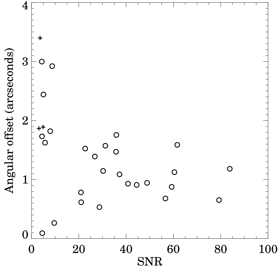
FIG. 3.— Positional offsets between the centroids of point sources detected at 70\mu\text{m} and the 2MASS position (after correcting for proper motion due to the time difference between the observations) as a function of the signal-to-noise ratio measured at 70\mu\text{m} . For symbols see the caption of Fig. 1. Apart from HD 14691, HD 48391 and HD 86146 all of the detected sources exhibit excess emission at 70\mu\text{m} .
