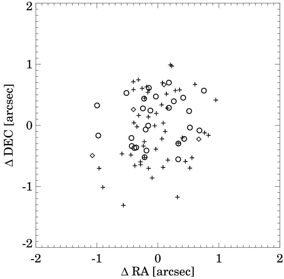
FIG. 1.— Offset between the source positions at 24\mu\text{m} and the 2MASS position (after correcting for proper motion due to the time difference between the observations). Plus signs indicate stars with pure photospheric emission, circles show stars exhibiting excess at one or more MIPS wavelengths, while targets surrounded by bright extended nebulosity at 24\mu\text{m} and/or 70\mu\text{m} are represented by diamonds. The distributions of the offsets for stars with and without excess are in agreement within their formal uncertainties.
