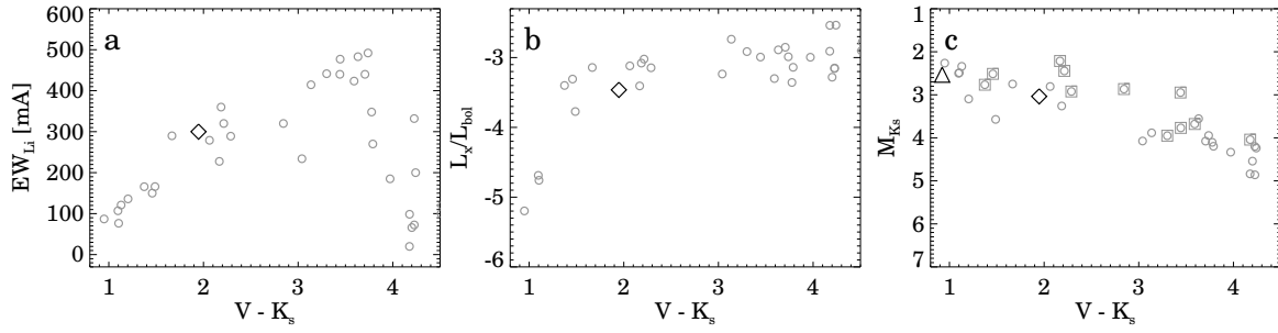
FIG. 10.— a) The distribution of Li equivalent widths as a function of V - K_s color indices. b) The distribution of fractional x-ray luminosities as a function of V - K_s color indices. c) Color-magnitude diagram. Grey circles represent the known members of the \beta Pic moving group. Grey squares represent binary stars in the CMD. The black diamond represents BD+45° 598, the black triangle shows HD 15745.
