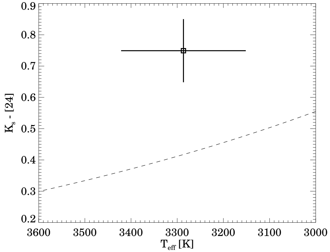
FIG. 13.— K_s -[24] color versus the effective temperature. The square shows the position of HD 113337B, the dashed line represents the locus of stellar photospheric colors determined by Gautier et al. (2007).
