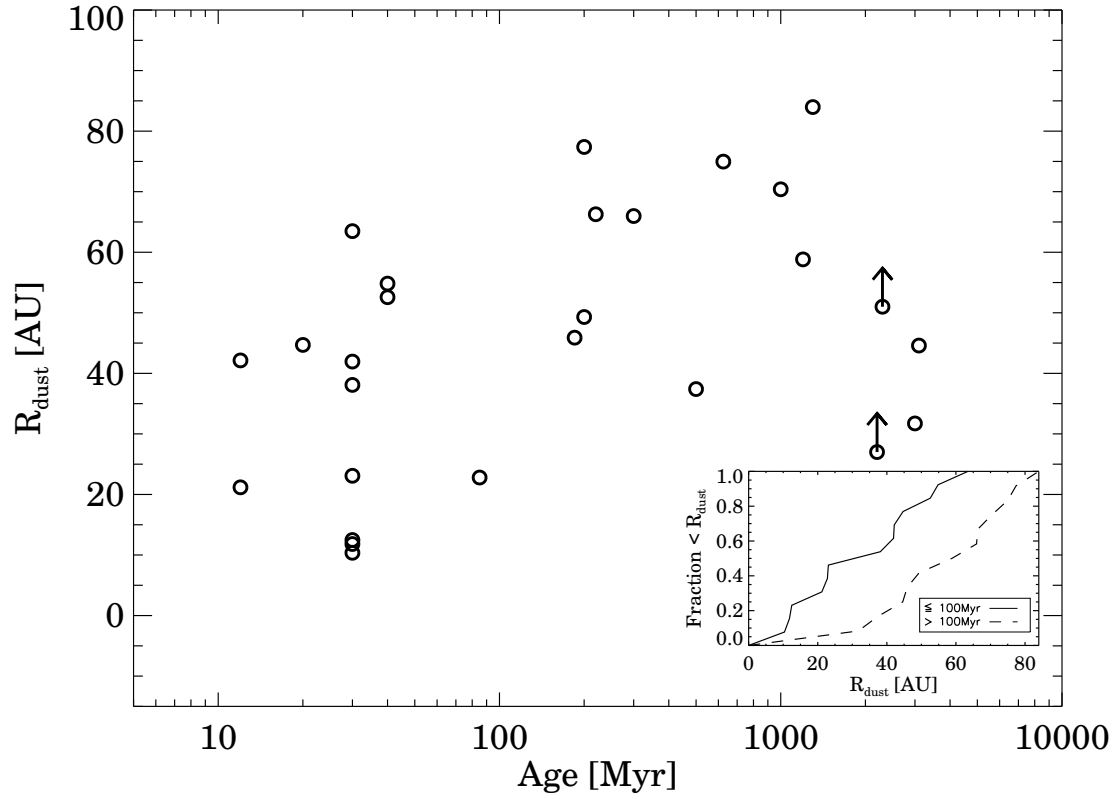
FIG. 16.— Derived dust radii as a function of age. Typical formal uncertainties in the derived disk radii range from 5% to 20%. The inset shows a comparison between the cumulative distribution of disks' radii around stars with age < 100 Myr and stars with age > 100 Myr (disks with lower limits for radius are not included). The inset does not cover any symbols.
