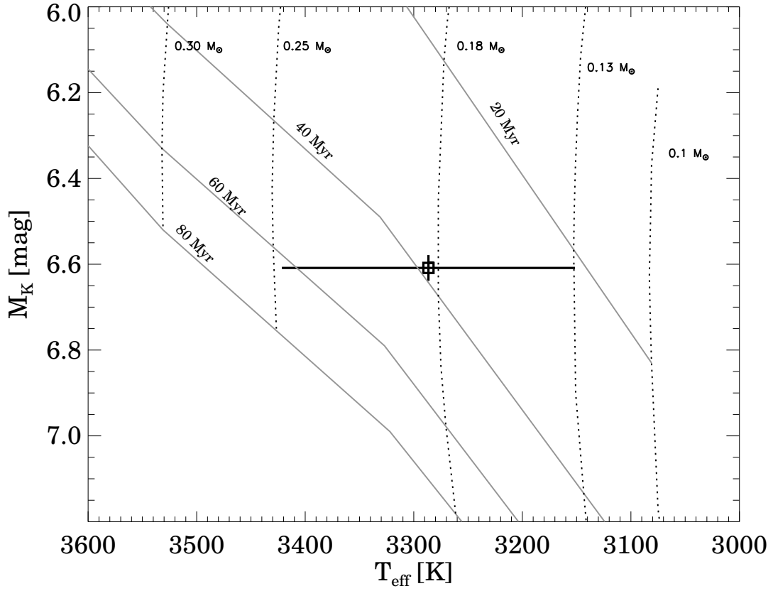
FIG. 12.— H-R diagram for HD 11337B. The effective temperature of the star and its uncertainty are estimated based on spectral class information (1 subclass uncertainty is assumed), the absolute magnitude in K-band is computed by assuming that it is located at the same distance as the primary component. Mass tracks and isochrones computed by Siess et al. (2000) for the evolution of stars with solar metallicity are overplotted. Based on these evolutionary tracks we find the age of the HD 11337B to be 40 \pm 20 Myr and the mass is \sim 0.13 - 0.25 M_{\odot} .
