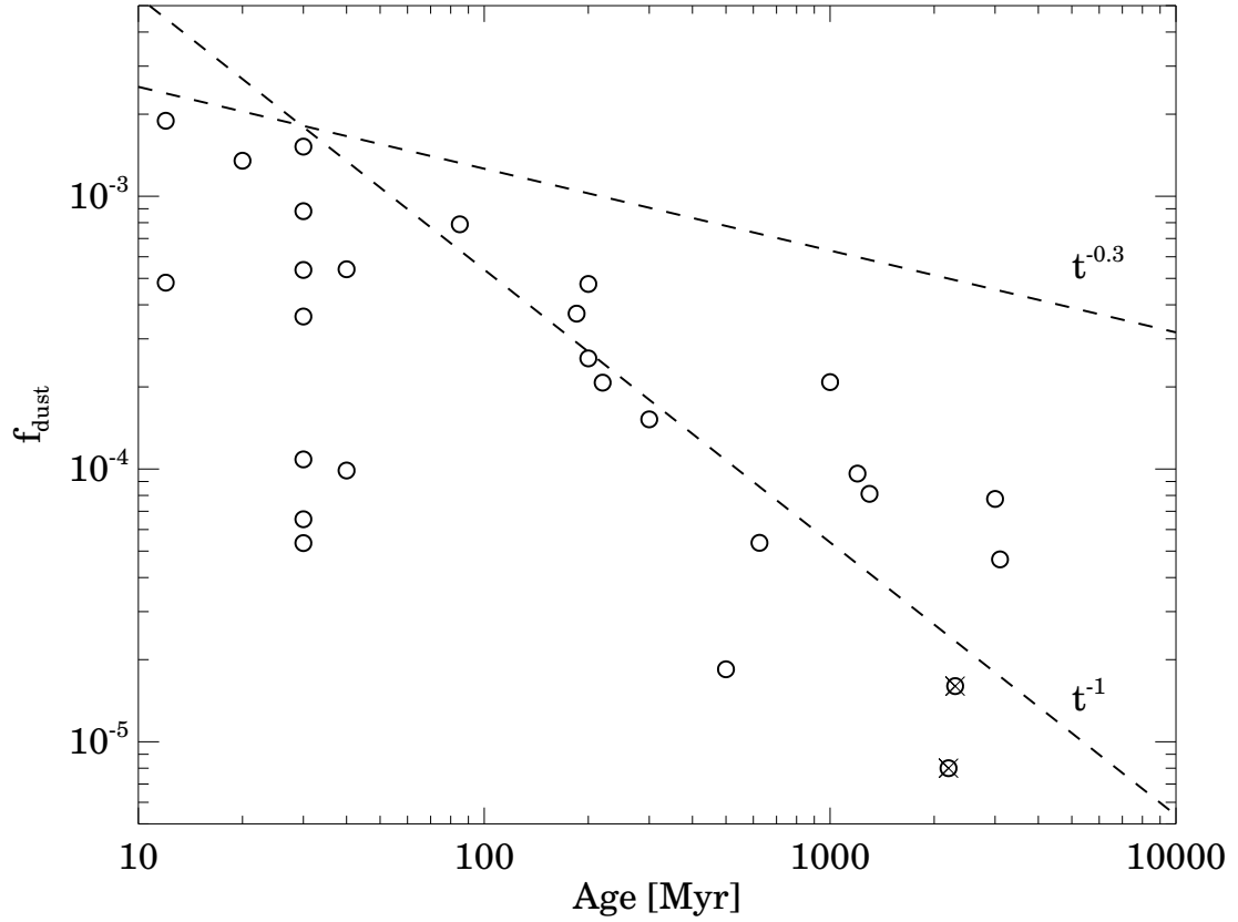
FIG. 15.— Fractional luminosity of the infrared excess as a function of age. Typical uncertainties in fractional luminosity range from 0.02 dex to 0.12 dex. Crosses mark disks where the excess emission was measured only in one IR band, thus they have less reliable fractional luminosities. Models of debris disk evolution predict that the decay of fractional luminosity is proportional to t^{-\alpha} where \alpha ranges between 0.3 and 1.0 (see Sect. 5.4). For comparison with our data, we plotted the two extremes of the evolutionary models with arbitrary normalization (dashed lines). The distribution of the data points, in particular their upper envelope, seems to suggest a decay rate halfway between the two extremes.
