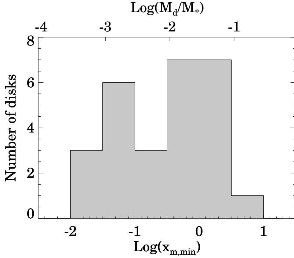
FIG. 18.— Histogram of the minimum x_{m,\min} values that are required for the observed disk to become self stirred in t < t_{\text{system}} . Initial disk-to-star mass ratios corresponding to the computed x_{m,\min} are indicated on the top of the graph (Sect. 5.5).
