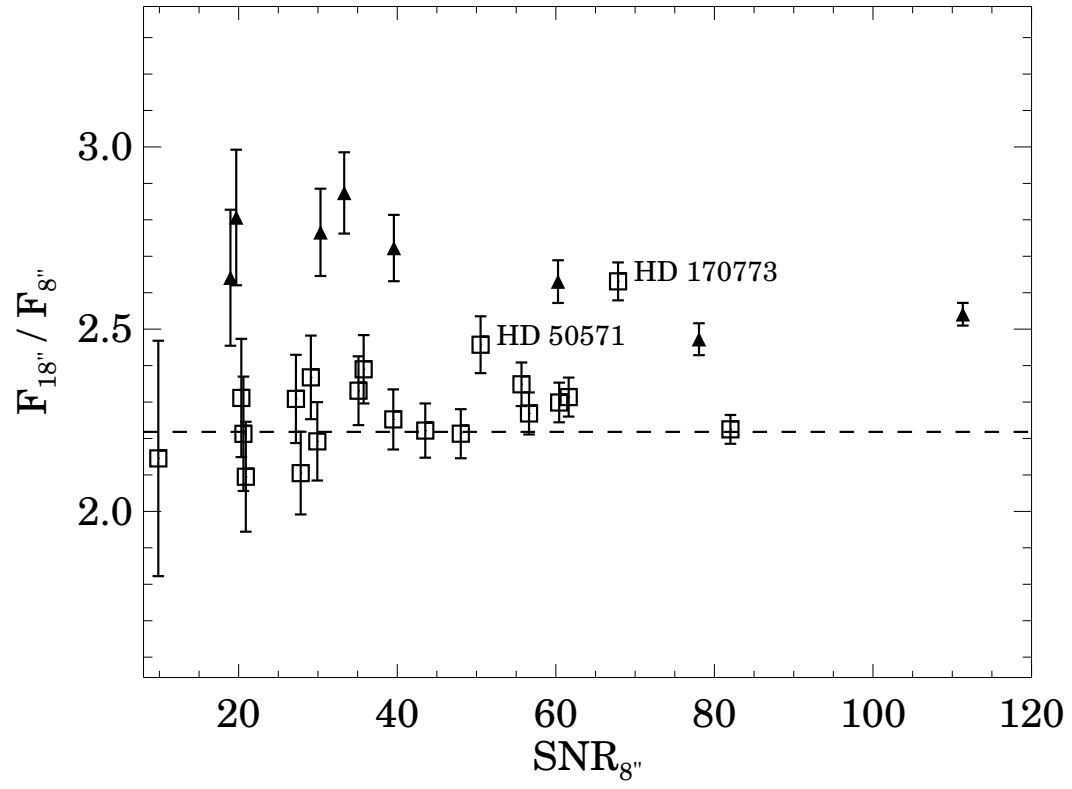
FIG. 7.— The ratio of the flux density measured in apertures with radii of 18'' and 8'' as a function of the SNR obtained in the smaller aperture. Squares indicate our stars that exhibit excess at 70\mu m , triangles correspond to debris disks (HD 10647, HD 38858, HD 48682, HD 105211, HD 115617, HD 109085, HD 139664, HD 207129) that found to be marginally resolved at this wavelength by Bryden et al. (2006).
