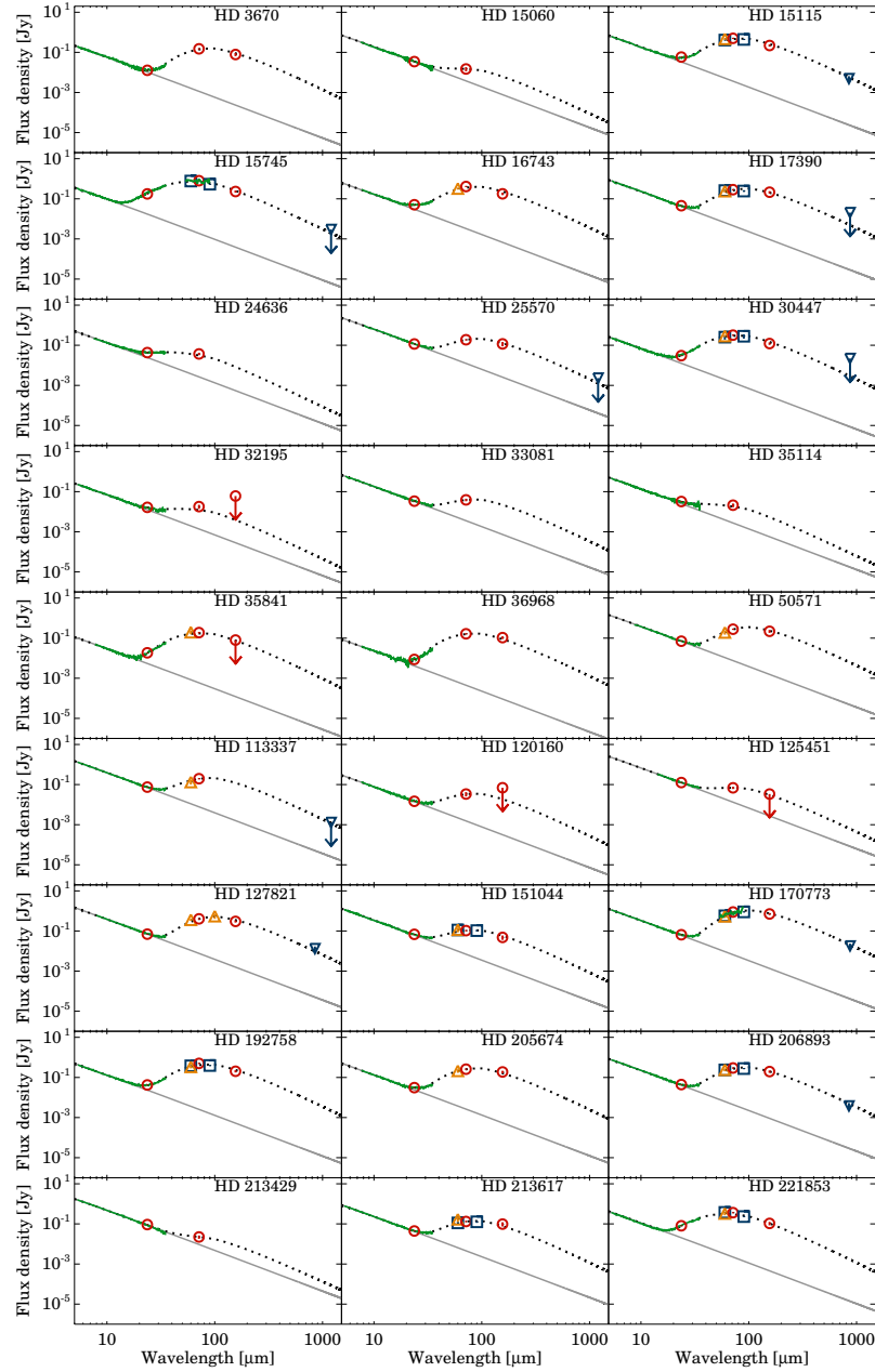
FIG. 9.— Spectral energy distributions for stars exhibiting IR excess in our sample. The different symbols represent the following photometric data - red circles: MIPS, blue squares: ISOPHOT, yellow triangles: IRAS, blue upside down triangles: submillimeter/millimeter observations. The IRS and MIPS SED spectra are displayed with green lines. The photospheric models and the disk models are shown by solid grey lines and dotted black lines, respectively. For HD 15115, HD 15745, HD 16743, HD 30447 and HD 192758 the two-component disk models are displayed.
