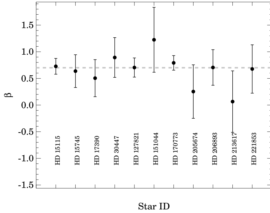
FIG. 8.— Derived \beta values for some selected disks (see Sect. 4.4).
