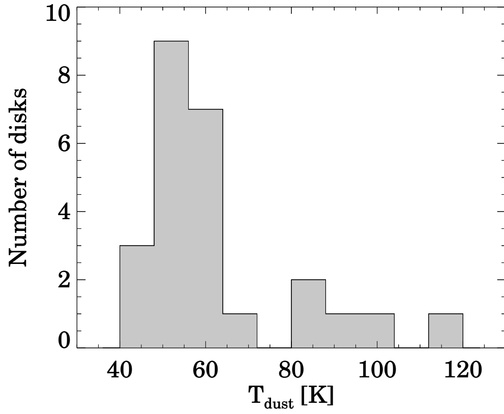
FIG. 14.— Histogram of the derived dust temperatures. In those cases where the presence of two separated dust rings are assumed only the temperature of the colder ring has been taken into account.
