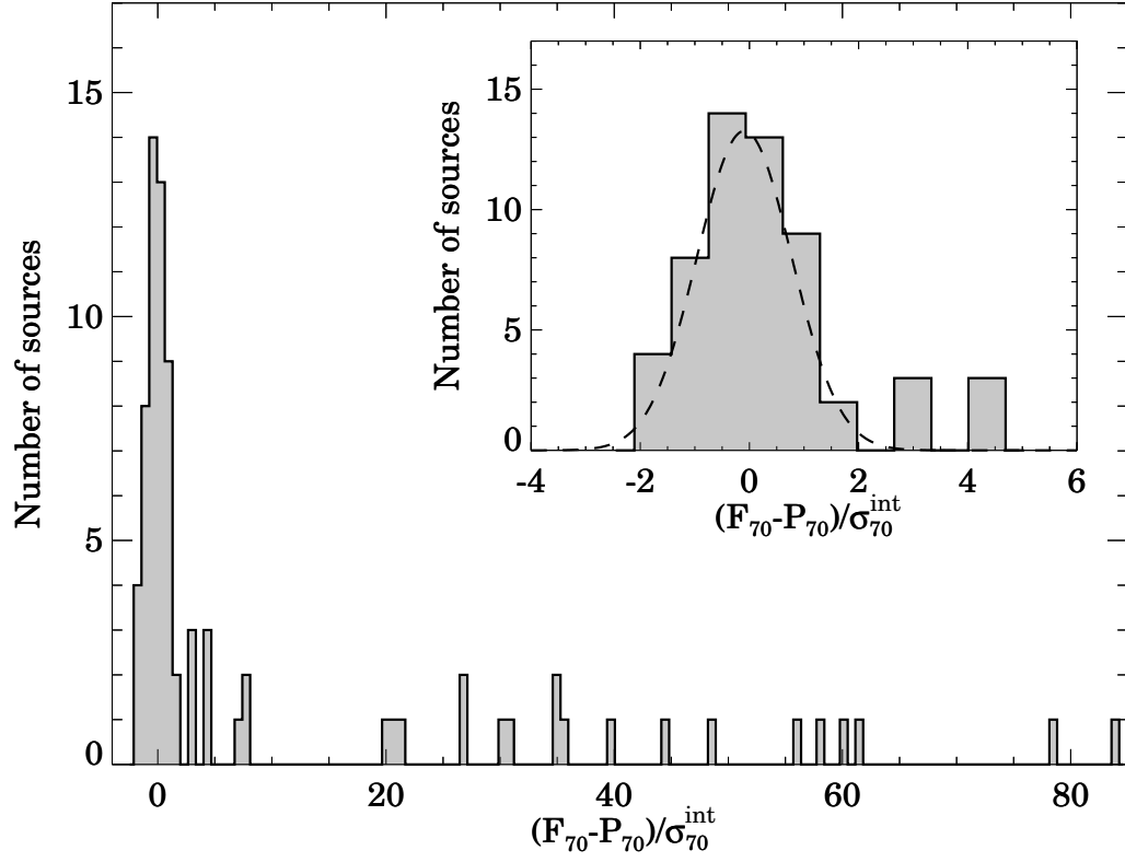
FIG. 4.— Histogram of the significances of the differences between the measured and predicted photospheric flux densities, defined as (F_{70} - P_{70})/\sigma_{70}^{\text{int}} , for targets measured at 70\mu\text{m} . Small panel: a zoom for the peak at zero. A Gaussian fit to the peak provides a mean of -0.09 and a dispersion of 0.87 , in good agreement with the expectations.
