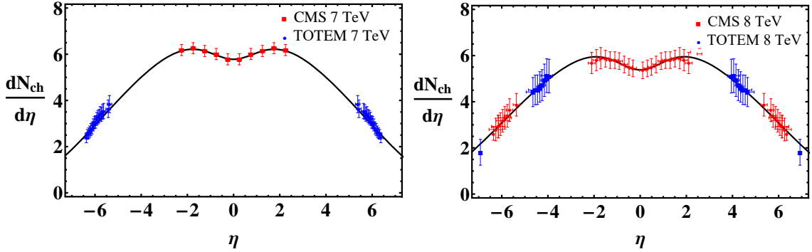
Figure 4: Left: Charged particle \frac{dN}{d\eta} distributions from CMS [51] and TOTEM [67] at 7 TeV fitted with the result of our relativistic hydrodynamical solution described in this paper, with \lambda = 1.076 . Right: Charged particle \frac{dN}{d\eta} distributions from CMS and TOTEM 8 TeV data of Ref. [62, 68] fitted with our results, with \lambda = 1.066 .
