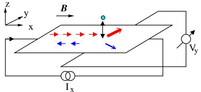
FIG. 2: (color online) Proposed measurement setup for experimental investigation of the Hall-like effect if an impurity plane is present in the sample at a finite distance from the 2DEG plane. The short horizontal red (blue) arrows in the figure represent spins parallel (antiparallel) to the polarizing magnetic field \mathbf{B} .
