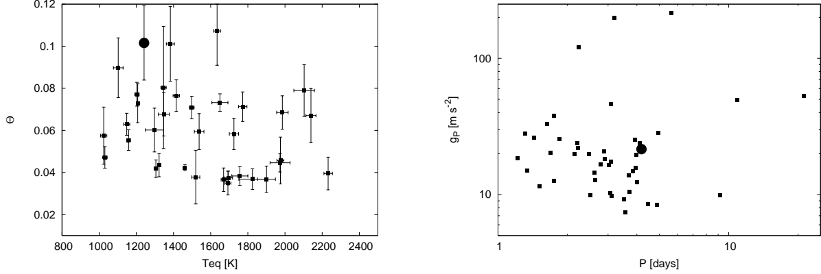
FIG. 6.— (a): Saffronov number vs. equilibrium temperature for the known transiting extrasolar planets. XO-5b is marked with a larger dot and it is located at the upper envelope of the Class I distribution of planets (XO-5b > 0.05 ). (b): Surface gravities as the function of the orbital period for the known extrasolar planets. With its relatively high surface gravity and orbital period, XO-5b falls slightly off the main distribution.
