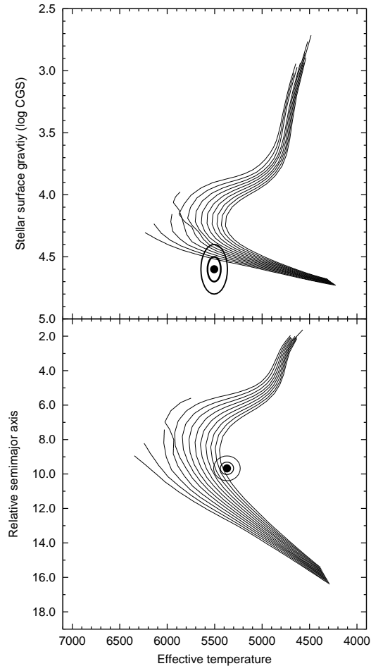
FIG. 5.— Stellar evolution isochrones from the Yonsei-Yale models, corresponding to ages between 2 and 14 Gyr (in steps of 1 Gyr), as a function of both surface gravity (top) and normalized semimajor axis a/R_* (bottom). In the top panel the isochrone metallicity ( [\text{Fe}/\text{H}] = +0.16 ), spectroscopic surface gravity, and temperature are from our initial SME analysis, the latter two shown with 1\text{-}\sigma and 2\text{-}\sigma confidence ellipsoids. In the lower panel the metallicity ( [\text{Fe}/\text{H}] = +0.05 ), temperature, and a/R_* are from the iterative analysis described in the text. Note that the latter quantities result in a significantly different evolutionary state for the star.
