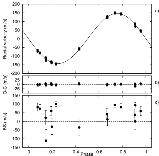
FIG. 3.— (a) Radial-velocity measurements from Keck for XO-5, along with our orbital fit (see § 5). The center-of-mass velocity \gamma and the correlation correction for the bisector span variations has been subtracted. (b) Phased residuals after subtracting the orbital fit (also see § 5). The rms variation of the residuals is about 4.6 \text{ m s}^{-1} . (c) Bisector spans (BS) for 16 of the Keck spectra (including the iodine-free template). Note that the scales of the panels are the same.
