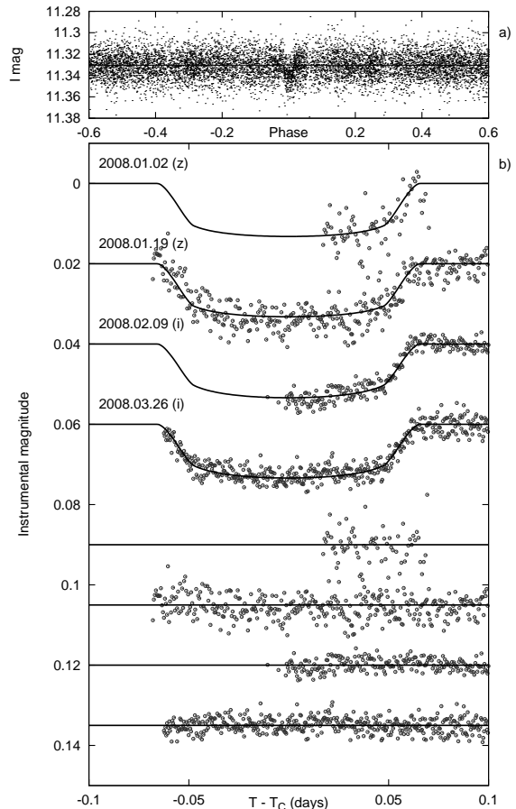
FIG. 1.— (a:) The light curve of XO-5 with all 14290 points taken in the I band, by the telescopes HAT-6, HAT-7, HAT-9 and WHAT. The light curve is folded with the period of P = 4.187757 \pm 0.000011 days (which is the result of the fit described in § 5). The superimposed curve shows the best fit model, neglecting limb darkening. (b:) Unbinned instrumental Sloan z band and i band follow-up transit photometry light curves acquired with KeplerCam on the FLWO 1.2 m telescope on 2008 January 2 ( N_{\text{tr}} = 0 , z band), January 19 ( N_{\text{tr}} = 4 , z band), February 9 ( N_{\text{tr}} = 9 , i band) and March 26 ( N_{\text{tr}} = 20 , i band). Superimposed are our best-fit transit models (§ 5).
