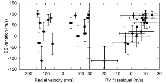
FIG. 4.— Bisector span variations as a function of the RV (left panel) and RV fit residual (right panel). The right panel shows the fit residuals when the correlation term was not included in the fit. Note that on the graphs the horizontal scales are not the same.
