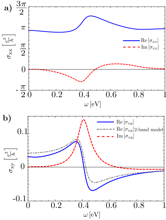
FIG. 6. (Color online) a) The real (blue solid line) and imaginary part (red dashed line) of the longitudinal optical conductivity \sigma_{xx} (in units of e^2/h ) given by Eq. (A9a). b) The real (blue solid line) and imaginary part (red dashed line) of the optical Hall conductivity \sigma_{xy} (in units of e^2/h ) calculated from Eq. (A9b), and the real part of \sigma_{xy} (gray dash-dot line) calculated from the two-band model according to Ref. 14. In both panels the chemical potential and temperature are zero, and the parameters are \Delta_T = 1 meV, \gamma_1 = 0.4 eV, \eta = 0.05 eV. (Note that our parameter \eta = 2\Gamma used in Ref. 15).
