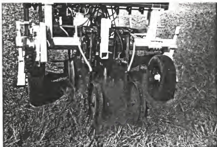
Figure 26. Test Plot at the Fort Hays Branch Agricultural Experiment Station.
