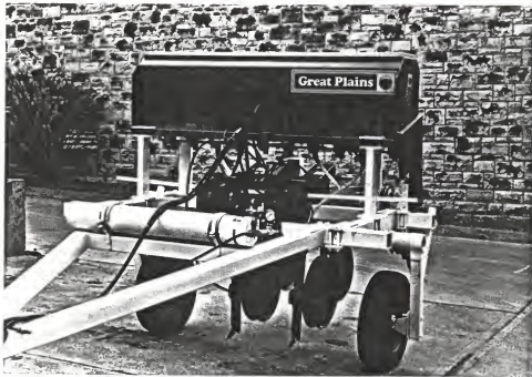
Figure 10. KSU Hoe Drill.
