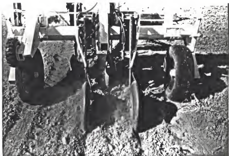
Figure 25. Test Plot at the Garden City Branch Agricultural Experiment Station.
