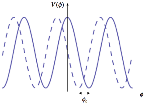
Figure 5.1: Original sine-Gordon potential (continuous line) and shifted potential (dashed line) under deformation.
