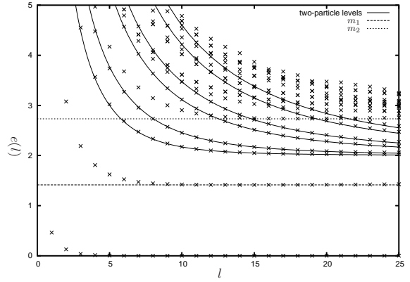
(b) Sector \mathcal{H}_3 of \mathcal{A}_6^{(1,2)-}
