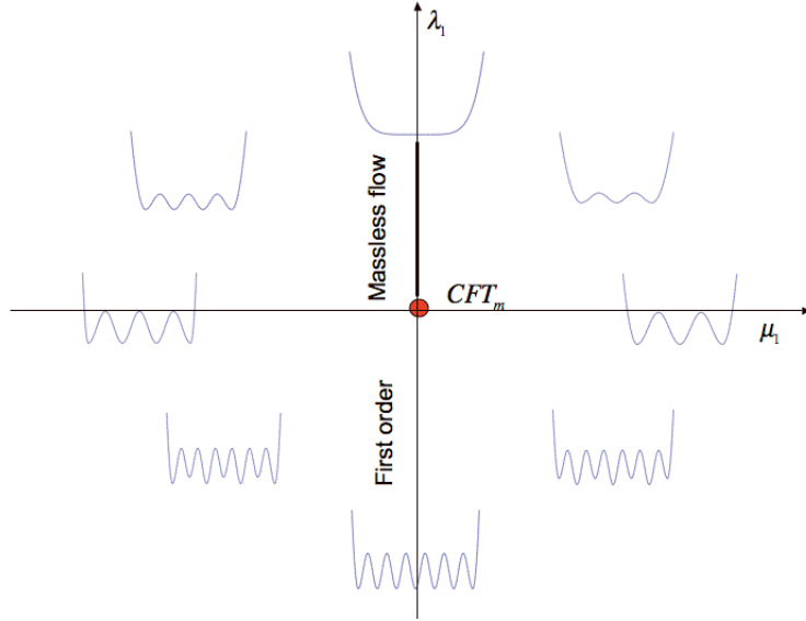
Figure 4.2: Evolution of the vacua structure of the \mathcal{A}_m^{(1)} theory in the plane of the couplings. This example refers to m = 8 .
