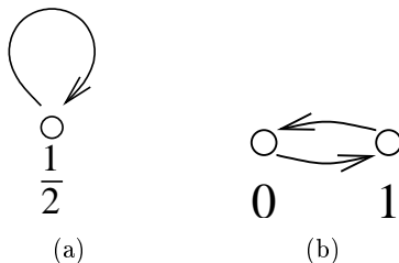
Figure 3.3: The two phases of the Ising model: (a) T > T_c ( \mathcal{A}_3^{(2,1)+} ) (b) T < T_c ( \mathcal{A}_3^{(2,1)-} )
