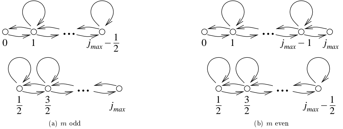
Figure 3.2: Adjacency rules for the kinks in \Phi_{1,2} perturbations ( j_{\max} = \frac{m-2}{2} )
