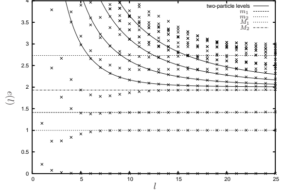
(b) Sector \mathcal{H}_2 of \mathcal{A}_6^{(1,2)\pm}
