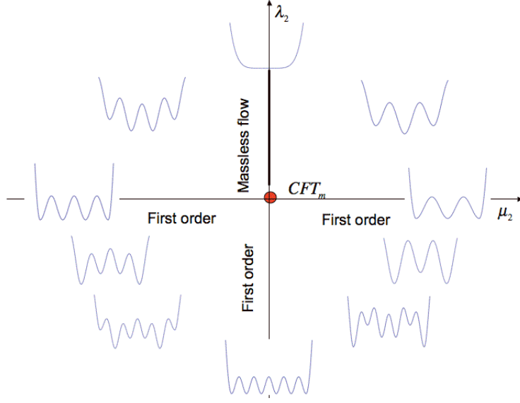
Figure 4.4: Evolution of the vacua structure of the \mathcal{A}_m^{(2)} theory in the plane of the couplings when m is odd. This example refers to m = 7 .
