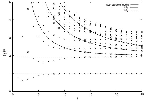
(a) Sector \mathcal{H}_3 of \mathcal{A}_6^{(1,2)+}
