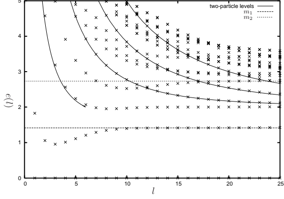
(a) Sector \mathcal{H}_1 of \mathcal{A}_6^{(1,2)\pm}
