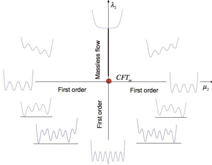
Figure 4.3: Evolution of the vacua structure of the \mathcal{A}_m^{(2)} theory in the plane of the couplings when m is even. This example refers to m = 8 .
