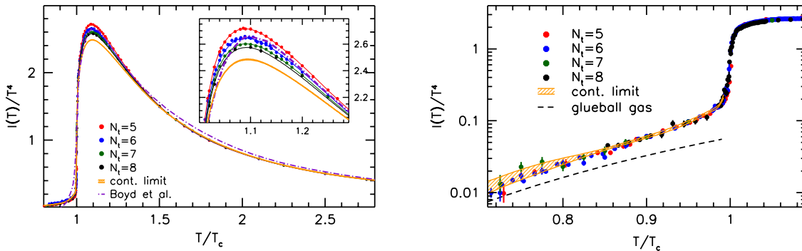
Figure 1: Left side. The trace anomaly calculated on 80^3 \times 5 , 96^3 \times 6 , 114^3 \times 7 and 64^3 \times 8 lattices. The continuum extrapolation makes use of the N_t^{-2} scaling of the Symanzik action. The data deviates from Boyd et al [5] especially close and below the transition. Right side. The trace anomaly in the confined phase measured on lattices with various lattice spacings and the continuum extrapolation (yellow band). The dashed line corresponds to the gluon gas contribution, estimated from the twelve lightest glueballs.
