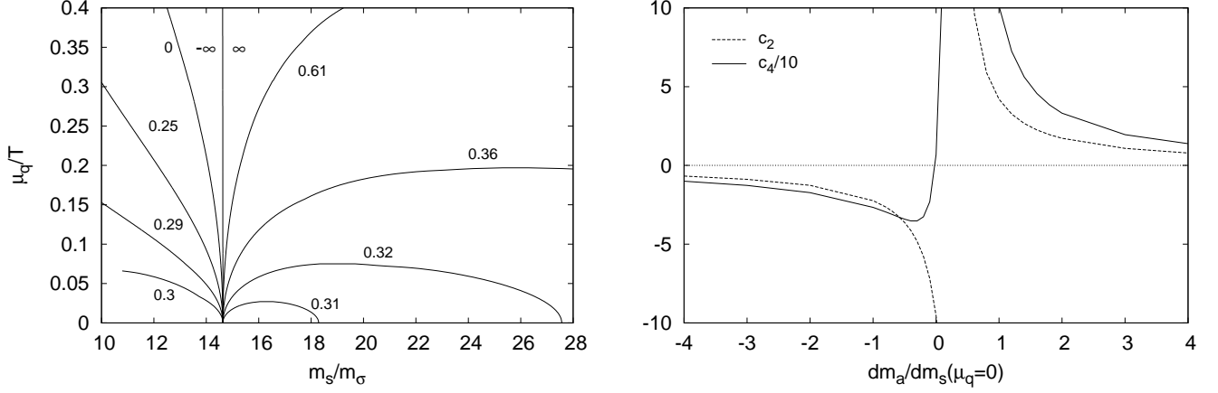
FIG. 5. Left panel: The m_s -dependence of the critical \mu_q/T obtained for u = 10 and g^2 = 3 . The labels on the curves indicate the value of dm_a/(dm_s)(\mu = 0) . Right panel: The first two coefficients of the Taylor expansion in Eq. (39).
