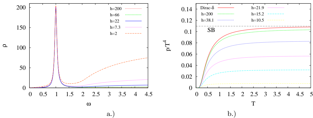
FIG. 3. a.) Spectral functions consisting of a single peak at m = 1 and \gamma = 0.05 , and a 2-particle cut with varying relative height starting at threshold m_{th} = 2 . h is the peak height of (9). The curves are rescaled to keep the quasiparticle peak unchanged. b.) The dependence of the pressure on the continuum height.
