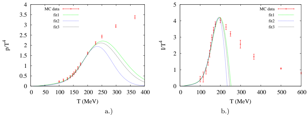
FIG. 5. Effect of the reduction of the number of degrees of freedom on the Hagedorn spectrum: a.) pressure, b.) interaction measure. The parameters of the fits is contained in I.
