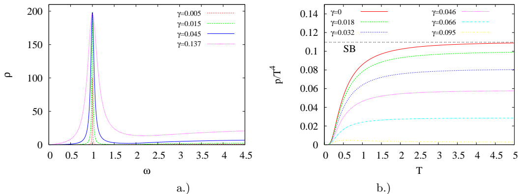
FIG. 2. a.) Spectral functions consisting of a single peak with different width parameters at m = 1 and a 2-particle cut starting at threshold m_{th} = 2 . The curves are rescaled for better visibility. b.) The width dependence of the pressure.
