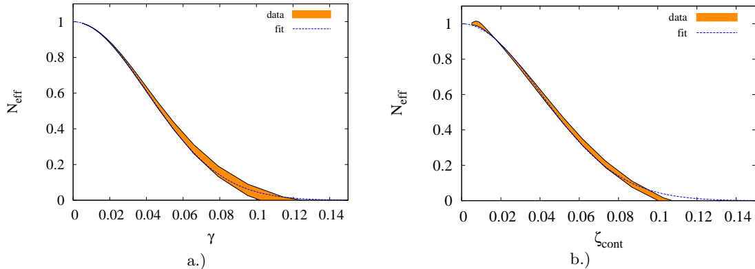
FIG. 4. Effective number of thermodynamical degrees of freedom in the studied temperature range, for a.) Scenario 1, b.) Scenario 2. The shaded regions represent temperature dependence of the definition. The fit functions were Gaussian.
