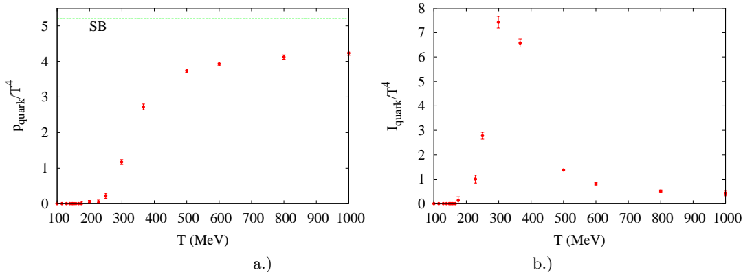
FIG. 6. The pressure and trace anomaly (interaction measure) of the QGP, according to our model predictions and MC data. SB means the asymptotic Stefan-Boltzmann limit.
