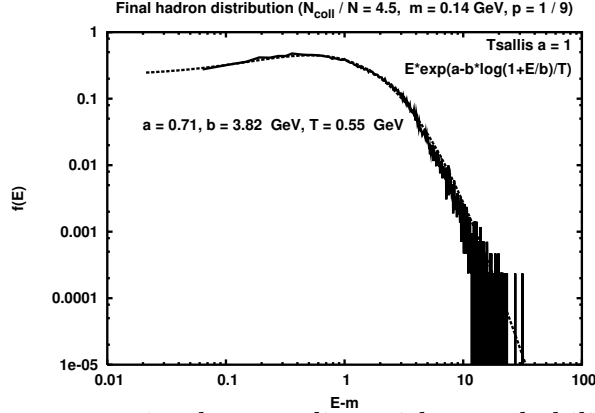
Figure 1. Pion spectrum emerging by sampling with a probability 1/9 from the NEBE parton cascade with massless partons.
