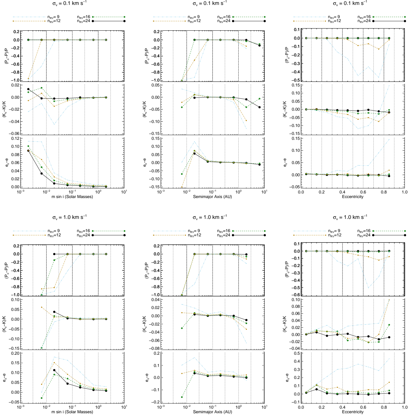
FIG. 13.— The recovered simulated systems binned by their recovered companion mass ( m \sin i ; left column), semimajor axis ( a ; center column), and eccentricity ( e ; right column). In each plot, the ordinates are the fractional error in period (top panel), fractional error in semiamplitude (middle panel), and error in eccentricity (bottom panel), where X_o indicates the recovered value of parameter with true value X . The top row of plots present the results using a base RV uncertainty of \sigma_v = 0.1 \text{ km s}^{-1} , and the bottom row shows \sigma_v = 1 \text{ km s}^{-1} . Cyan, tan, green, and black points (dash triple-dotted, dash dotted, dashed, and solid lines) are from simulations with 9, 12, 16, and 24 visits, respectively. The vertical dotted lines mark the bins used, and for any bin with < 3 stars, the point is excluded.
