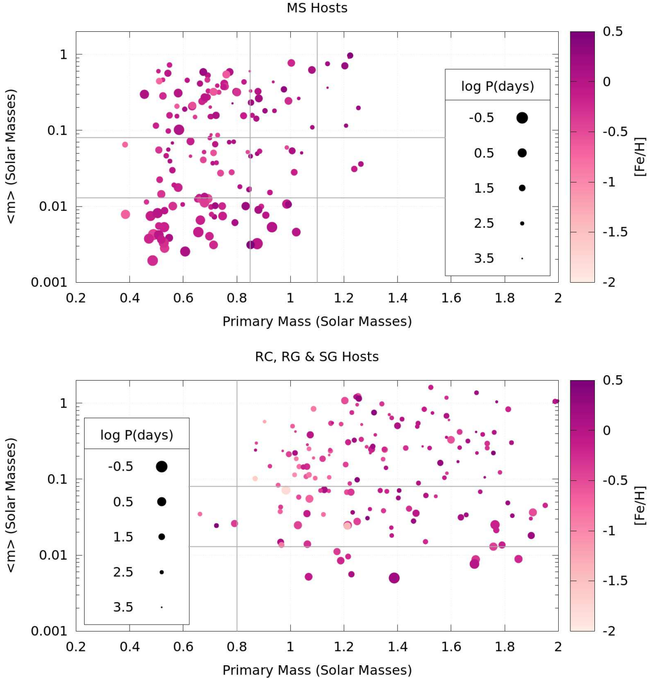
FIG. 7.— Modification of Figure 3 from Guillot et al. (2014), with M_* on the abscissa and maximum-likelihood companion-mass ( \langle m \rangle ) on the ordinate. Color represents the host stars’ metallicity, and point size represents the period of the companion in log days. Larger points here indicate companions that are more likely to be undergoing tidal interaction with their host star. Top Panel: Stars in the gold sample selected as MS stars. The vertical lines mark nominal G dwarfs ( 0.85 < M_*/M_\odot < 1.1 ), and the horizontal lines mark the BD mass regime ( 0.013 < \langle m \rangle/M_\odot < 0.08 ). Bottom Panel: Remaining stars in the gold sample with M_* < 2M_\odot . The horizontal lines again mark the BD mass regime, and the vertical line marks M_* = 0.8M_\odot . It would be a reasonable expectation that a giant star above this mass evolved from a star earlier than a G dwarf since solar-like stars lose about one third of their mass on the RGB.
