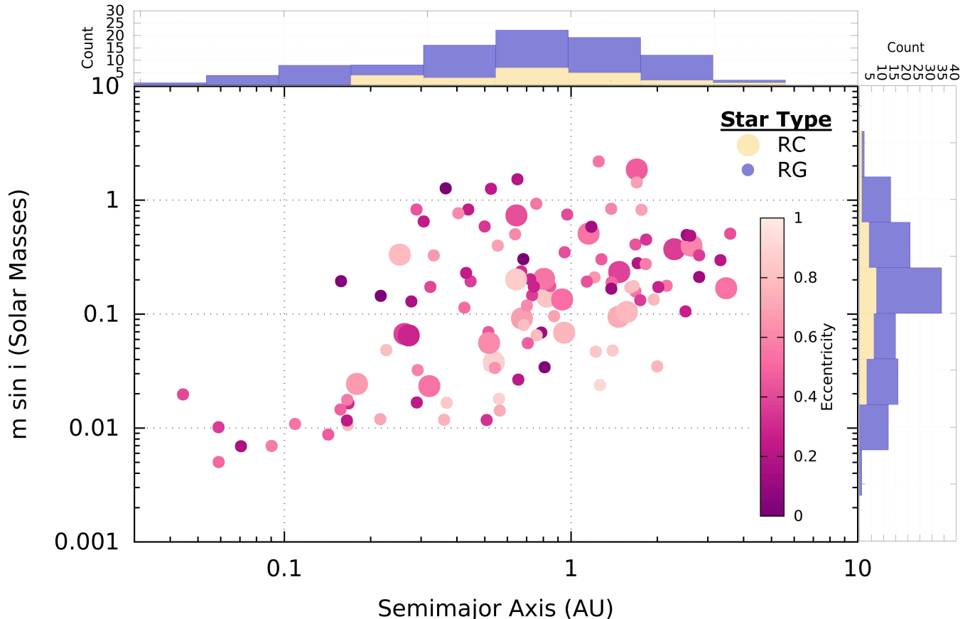
FIG. 9.— Orbital distribution of companion candidates to RC stars (large points) and RG stars with similar stellar parameters as this sample’s RC stars (small points). Minimum orbital semi-major axis in AU is on the abscissa and minimum companion mass in M_{\odot} is on the ordinate. Color again represents the orbital eccentricity of the companion. The panels above and to the right of main plot show the m \sin i and semi-major axis distribution for the RG comparison sample (purple histogram) and RC (gold histogram) hosts.
