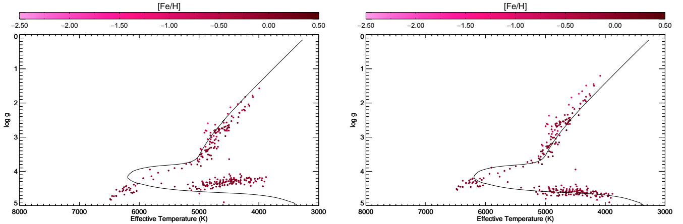
FIG. 3.— Spectroscopic HR diagrams of stars in the field of M67 observed by APOGEE with the stars’ T_{\text{eff}} and \log g as the abscissa and ordinate. The points are color-coded by host star metallicity. A 5 Gyr solar-metallicity isochrone is also included for comparison. Left Panel: Uncalibrated parameters (for both giants and dwarfs). Note the \log g is underestimated by \sim 0.5 for stars at T_{\text{eff}} \sim 4000 K. Right Panel: Calibrated parameters, with giants using the ASPCAP calibrated parameters and dwarfs adopting the \log g correction from Equation 3.
