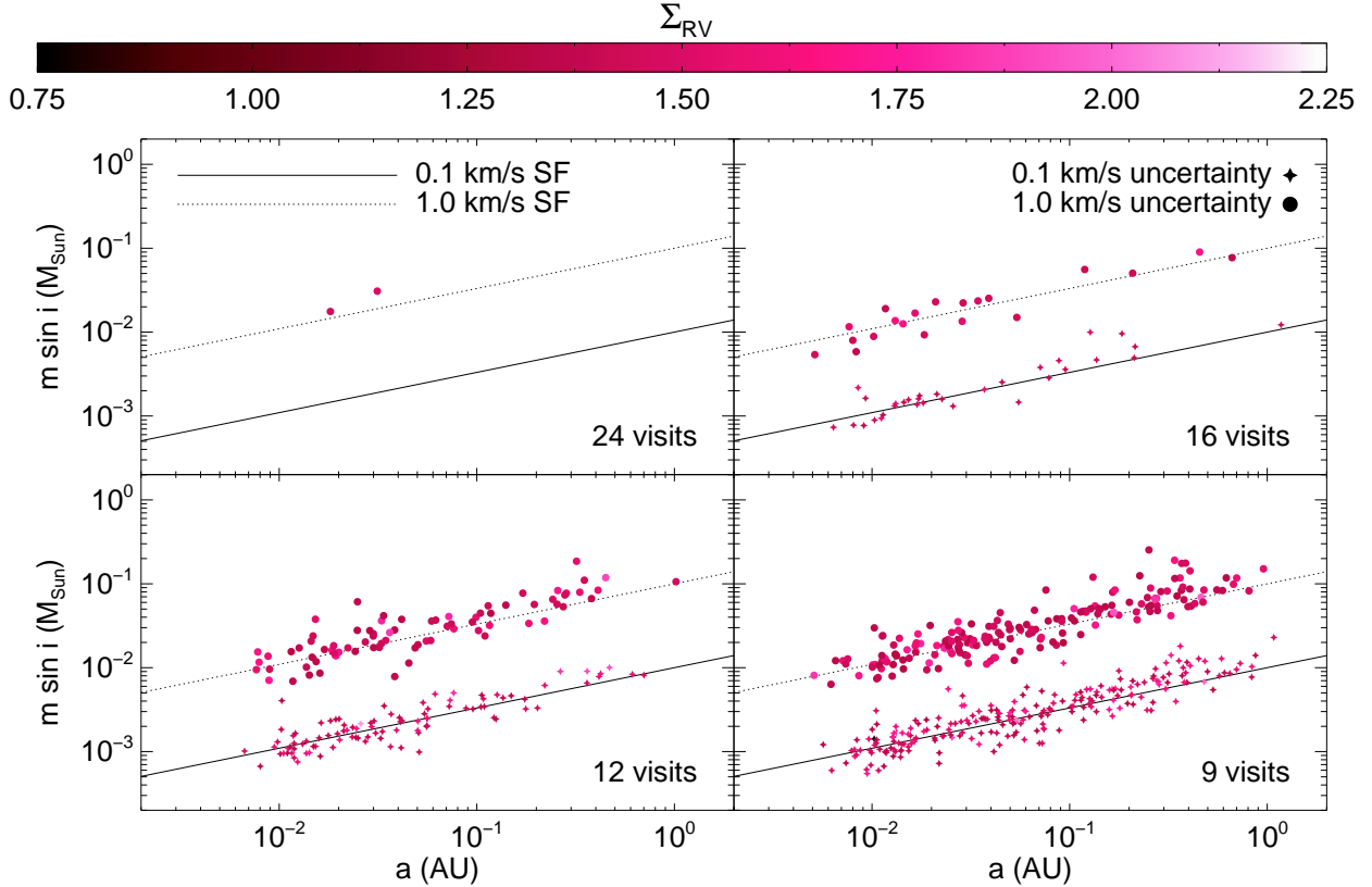
FIG. 11.— Distribution of false positive companions in recovered m \sin i - a space, with color representing the \Sigma_{RV} statistic (see equation 2). Each set of points (unique color and shape) is drawn from a sample of 18,000 simulated systems with 9 (bottom right panel), 12 (bottom left panel), 16 (top right panel), and 24 (top left panel) simulated RV measurements based on stellar jitter and random measurement error. Symbol shape indicates the uncertainty level used for the simulation, with circles indicating 1 \text{ km s}^{-1} and four-point stars indicating 0.1 \text{ km s}^{-1} uncertainties. The solid and dotted lines show the approximate sensitivity function (SF; see Equation A1) for 0.1 and 1 \text{ km s}^{-1} RV uncertainties. False positive signals such as these are removed from the sample via the velocity cut described in §3.1.2.
