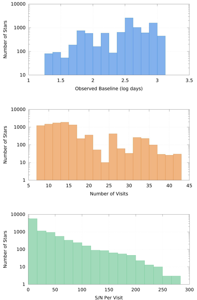
FIG. 1.— Top Panel: Distribution of the observed baseline for the 14,840 stars with at least eight visits. The median baseline for this set of stars is slightly over a year at 384 days. Middle Panel: Distribution of the number of visits to the same set of stars, with 13 being the median number of visits. Bottom Panel: Distribution of the average S/N per visit for the same set of stars, with a median S/N per visit of 12.2.
