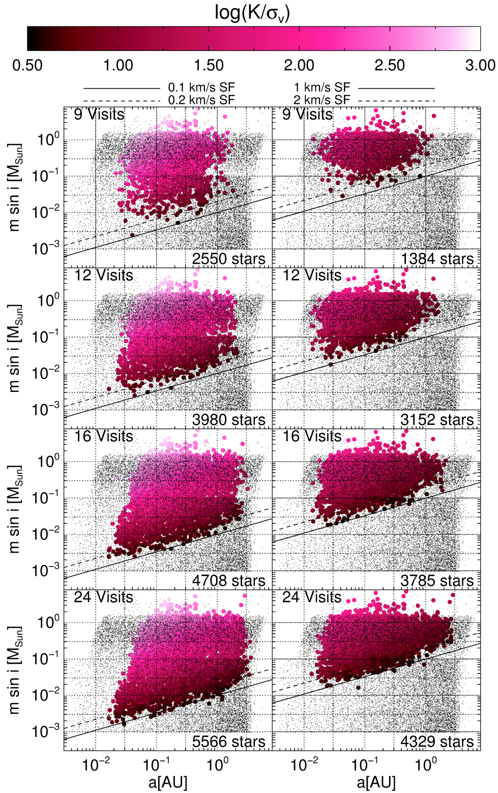
FIG. 12.— The grey dots are the locations of the 18,000 simulated systems in actual m \sin i - a space. The colored circles indicate the correctly recovered systems that were selected as candidates using the same metric as the “gold sample”, color-coded by recovered \log(K/\sigma) , with the number of systems correctly recovered indicated in the bottom right corner of each panel. The black solid and dashed lines mark the sensitivity function (SF; see Equation A1) for the baseline and twice the baseline RV uncertainties of 0.1 \text{ km s}^{-1} (left column) and 1.0 \text{ km s}^{-1} (right column) used by the simulations. The simulations presented here emulate stars with, from top row to bottom row, 9, 12, 16, and 24 visits.
