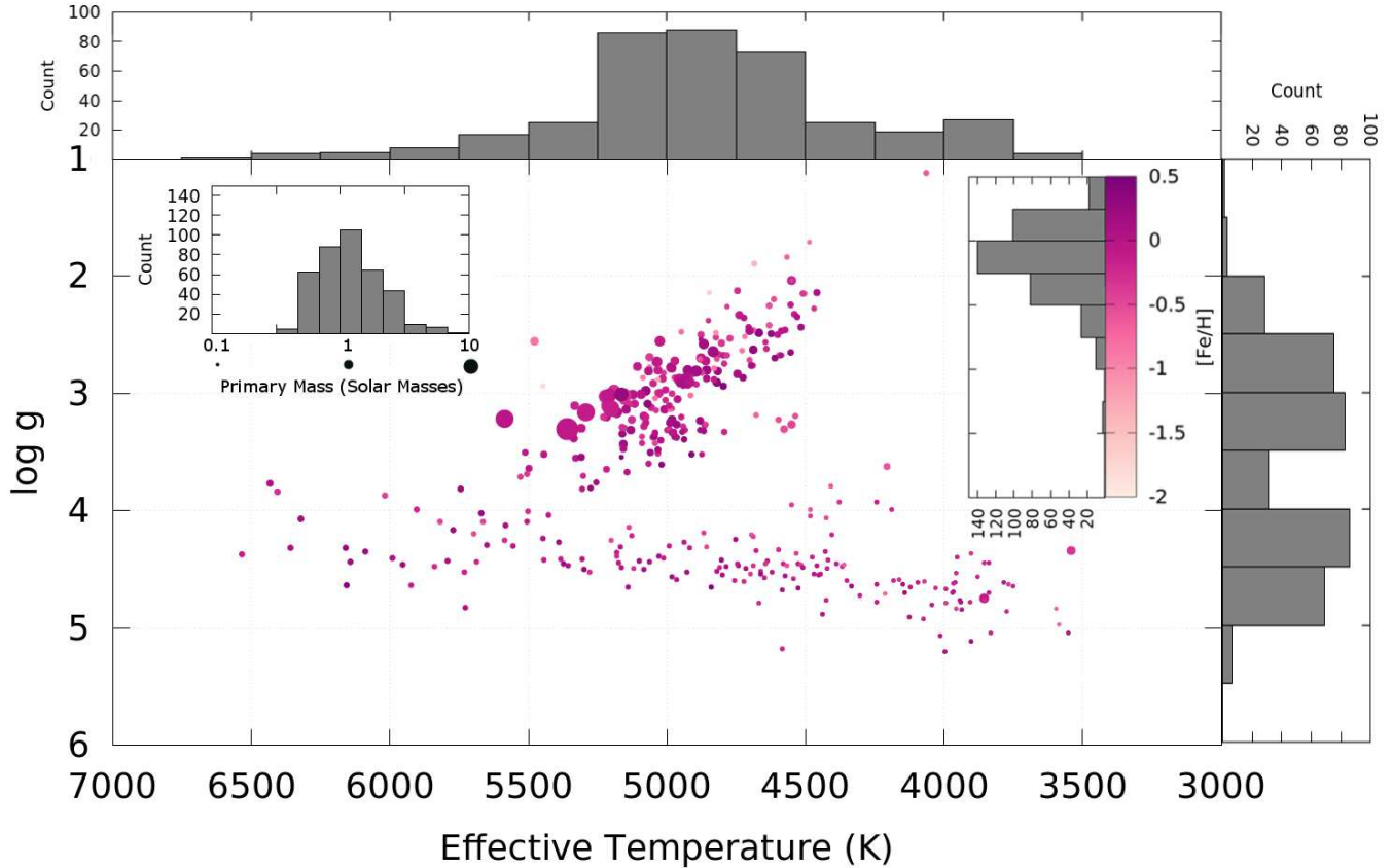
FIG. 8.— A spectroscopic HR diagram of the companion candidate hosting stars, with the host stars’ T_{\text{eff}} and \log g as the abscissa and ordinate. The points are color-coded by host star metallicity ( [\text{Fe}/\text{H}] ), and point size indicates the primary mass in Solar masses. The stars along the bottom of the figure are the dwarf stars, and stars along the line connecting (T_{\text{eff}}, \log g) = (5500 \text{ K}, 3.5) and (4000 \text{ K}, 1) are the giants. Histograms of the effective temperature ( T_{\text{eff}} , top panel), surface gravity ( \log g , right panel), metallicity ( [\text{Fe}/\text{H}] , inset with color bar), and primary mass (inset with size legend) of the host stars in this gold sample are also shown.
