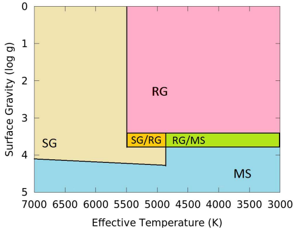
FIG. 4.— Classification scheme of Red Giant (RG), Subgiant (SG), and main-sequence dwarf stars (MS) in \log g - T_{\text{eff}} space. Red Clump (RC) and pre-main sequence stars (PMS) transcend these boundaries as they selected through alternate means. The areas labeled with SG/RG or MS/RG are regions where the star can be either classification depending on its metallicity. The upper left corner of this plot does not contain any stars in this sample, so the SG classification there is simply in place to cover the phase space.
