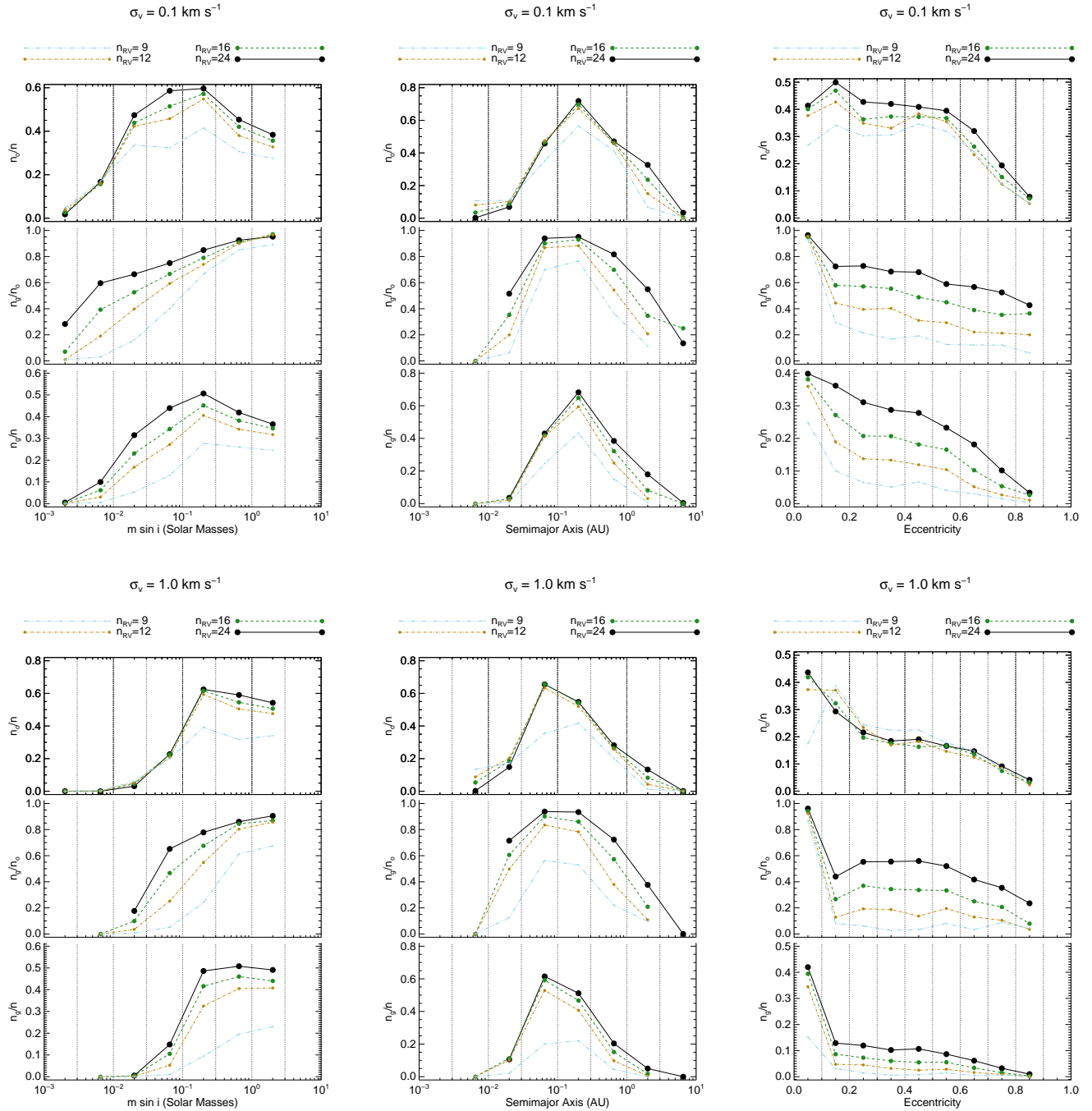
FIG. 14.— The same as Figure 13, except on the ordinate in each plot, the top panel shows the fraction of systems recovered in the bin, n_r , compared to the total number of simulated systems in the bin, n , the middle panel shows the fraction of systems recovered with correct orbital parameters ( P and K within 10% and e within 0.1), n_g compared to n_o , and the bottom panel shows n_g/n . Here a bin is excluded if the denominator of the ordinate is < 2 .
