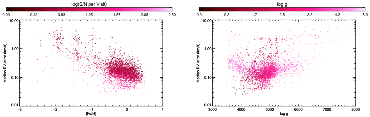
FIG. 2.— Left Panel: Precision of individual APOGEE visit RVs as a function of the metallicity ( [\text{Fe}/\text{H}] ) of the star with the color scale indicating the logarithm of the S/N per visit. Right Panel: Precision of individual APOGEE visit RVs as a function of the effective temperature ( T_{\text{eff}} ) of the star with the color scale indicating the surface gravity ( \log g ) of the star.
