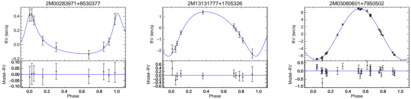
FIG. 5.— RV curves for a few example systems. In each plot, the top panel presents the phased RV measurements with a line showing the best fit model and the bottom panel shows the residuals of the fit. Similar figures are available online for every star in the gold sample (see Appendix B). Left Panel: A planetary-mass ( m \sin i = 4.60 M_{Jup} ) companion in a P = 41.3 day, a = 0.25 AU orbit with e = 0.566 , and K = 0.29 km s ^{-1} . This orbit has uniformity index (See §3.3.4) values of U_N = 0.886 and V_N = 0.737 . Middle Panel: A BD-mass companion ( m \sin i = 22.6 M_{Jup} ) companion in a P = 24.3 day, a = 0.15 AU orbit with e = 0.293 , K = 1.99 km s ^{-1} . This orbit has uniformity index values of U_N = 0.871 and V_N = 0.935 . Right Panel: Binary System with a m \sin i \approx 0.304 M_\odot secondary in a P = 184 day, a = 0.68 AU orbit with e = 0.004 , K = 7.11 km s ^{-1} . This orbit has uniformity index values of U_N = 0.937 and V_N = 0.869 .
