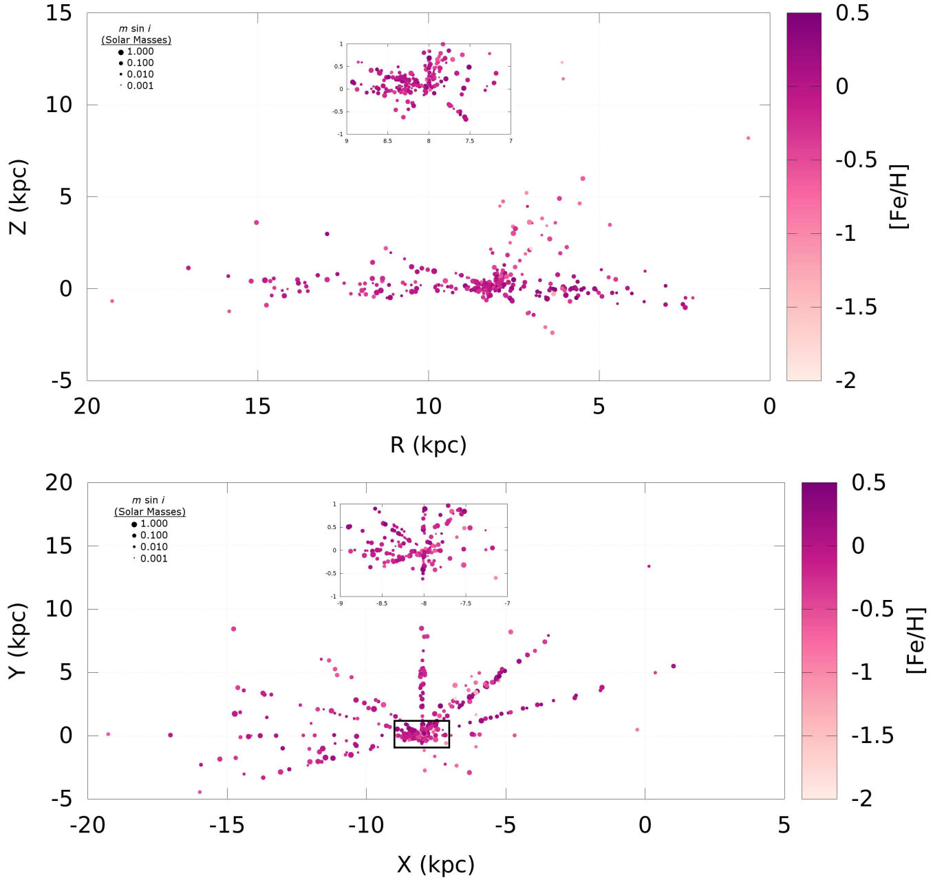
FIG. 10.— The Galactic distribution of companion candidate hosts in this catalog. Top Panel: Distribution in Galactocentric R and Z , where R is the radial distance from the Galactic Center, and Z is the height above the Galactic midplane. The color of the points indicates the metallicity ( [Fe/H] ) of host star, and the point size indicates m \sin i of the companion candidate orbiting the star. The inset panel shows a detailed view of the solar neighborhood, which is indicated by the black box in the main plot ( 7 \text{ kpc} < R < 9 \text{ kpc} , |Z| < 1 \text{ kpc} ). Bottom Panel: Distribution in Galactocentric X and Y rectilinear coordinates, where (X, Y) = (0, 0) and (-8, 0) kpc are the locations of the Galactic Center and the Sun respectively, and Y > 0 is in the direction of the Sun's orbit. The color and size of the points indicate the same data as they do in the top panel. Again, the inset panel shows a detailed view of the solar neighborhood, which is indicated by the black box in the main plot ( 7 \text{ kpc} < X < 9 \text{ kpc} , |Y| < 1 \text{ kpc} ).
