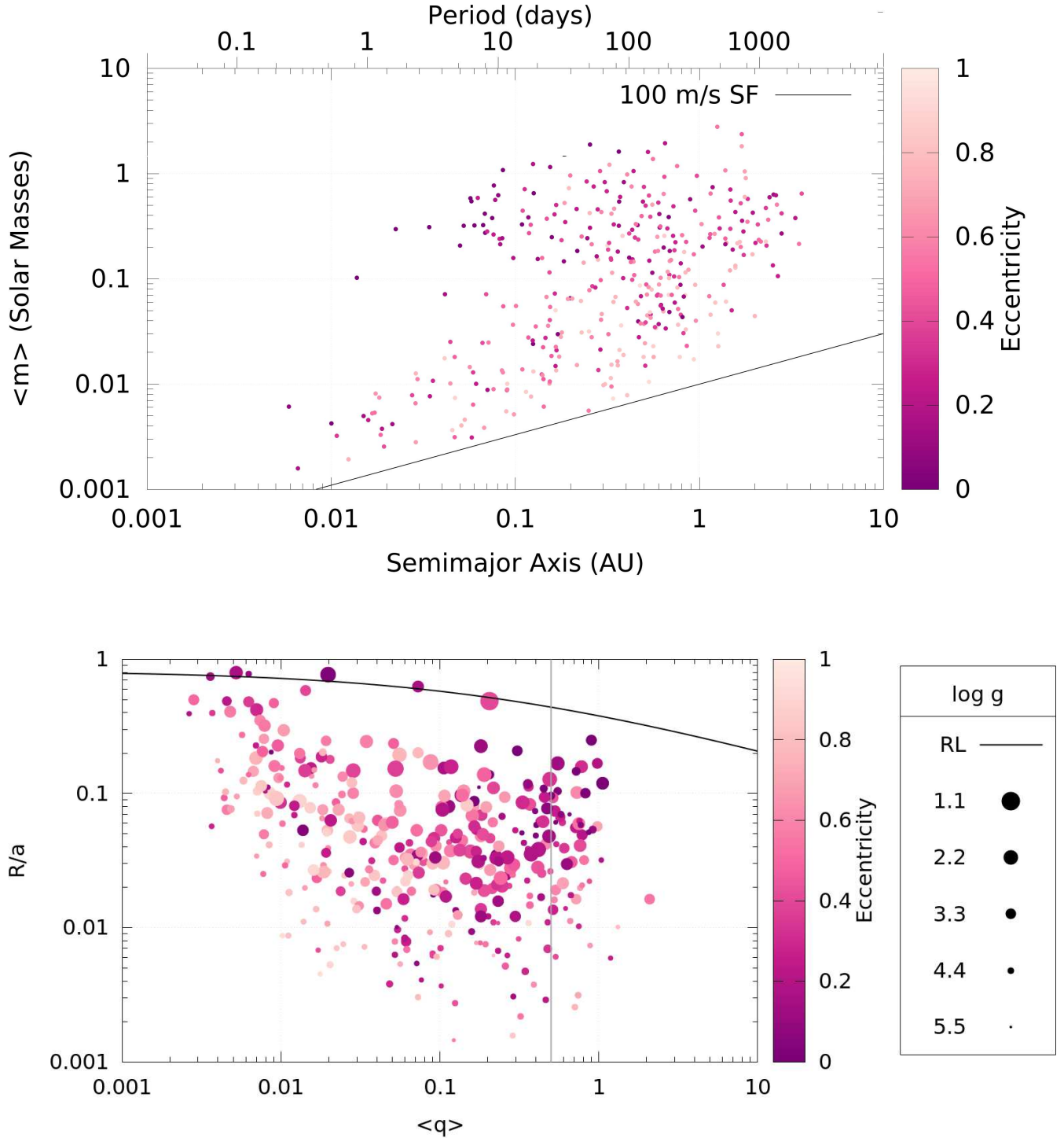
FIG. 6.— Top Panel: Orbital distribution of companion candidates in the 382-star gold sample with minimum orbital semi-major axis ( a ) in AU on the abscissa and maximum-likelihood companion mass ( \langle m \rangle = (4/\pi)m \sin i ) in M_{\odot} on the ordinate. The top horizontal axis gives the approximate period for the companion in days as well. Color represents the orbital eccentricity of the companion, with dark magenta representing circular orbits. The black line is the sensitivity function (SF; Equation A1) for 100 \text{ m s}^{-1} RV precision. Systems below this line would generally be undetectable by APOGEE. Bottom Panel: Orbital distribution of companion candidates with \langle q \rangle = \langle m \rangle / M_{\star} on the abscissa, and R_{\star}/a on the ordinate. Color again represents eccentricity, and point size indicates the surface gravity ( \log g ) of the host. The grey vertical line marks systems with \langle q \rangle > 0.5 , and the black line across the top of the panel indicates the Roche limit (RL; Equation 31) of the host star.
