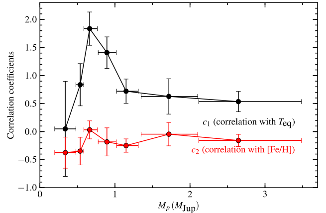
FIG. 7.— The correlation between planet radius, equilibrium temperature and metallicity are plotted. For each mass bin of size 20, we calculate the correlation coefficients c_1 and c_2 (Equation 1). The vertical error bars are derived from bootstrapping the sample. The horizontal error bars show the extent of each mass bin.
