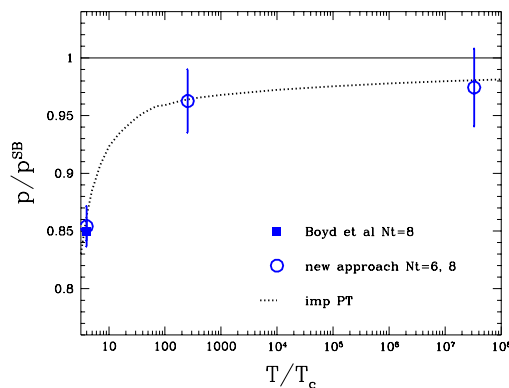
Figure 5: The pressure, normalized to its Stefan-Boltzmann value, as a function of the temperature obtained by our new technique. Results with smaller discretization errors ( N_t = 8 , blue circles), seem to fit improved perturbation theory, and also reproduce results obtained by the standard method at lower temperatures. At the highest temperature, 3 \cdot 10^7 \cdot T_C , the pressure (within its statistical uncertainty) is consistent with the Stefan-Boltzmann limit.
