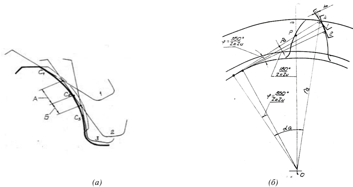
Fig. 4 – Wheel teeth precutting: a – a tooth of hob cutter with a prominence; b – a wheel tooth machined with \Delta allowance: h_n – the prominence height, a_0 – the angle of original profile, a_n – the angle of prominence profile
