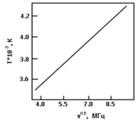
Fig. 1.6 - Dependence of the HFFD temperature on the field frequency
