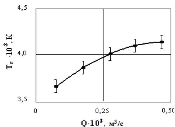
Fig. 1.11 - Dependence of the gas temperature of the HFFD in air on the gas pumping rate
