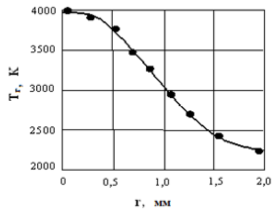
Fig. 1.9 - Radial distribution of gas temperature HFFD in air
