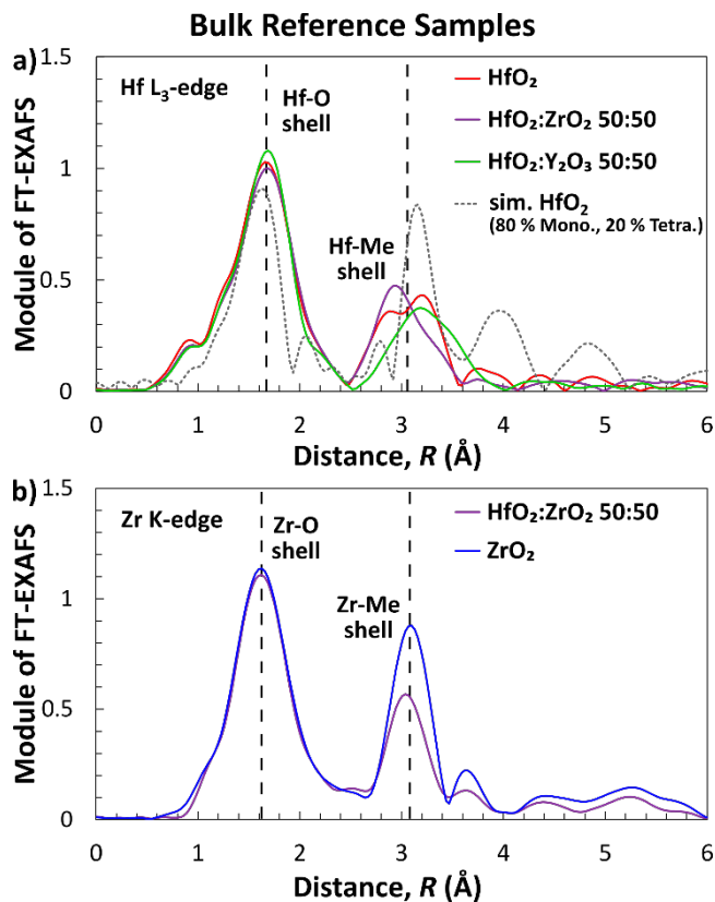
Figure 5. (a) Hf L_3 -edge and (b) Zr K-edge FT-EXAFS for \text{HfO}_2 , \text{Hf}_{0.5}\text{Zr}_{0.5}\text{O}_2 , \text{Hf}_{0.5}\text{Y}_{0.5}\text{O}_{2-y} , \text{ZrO}_2 powders. For the Hf L_3 -edge a theoretical spectrum of a mixture of 80 % monoclinic and 20 % tetragonal phase is provided (Please note that the amplitudes at higher R values are more pronounced as explained in the beginning of section 2). The vertical dashed lines are provided just for guidance to highlight the changes between the main peaks of the Me-O and Me-Me coordination shells. Note that the distances do not correspond to the real distances due to phase shift of the photoelectron. Distances for Hf and Zr are not comparable as this phase shift is different for Hf and Zr. However, the distances of the respective Hf or Zr edges can be compared between Figure 5 and Figure 9.
