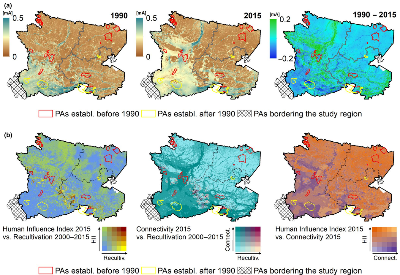
FIGURE 4 (a) Changes in landscape connectivity between 1990 and 2015. (b) Human influence index (left) and connectivity (middle) in relation to recultivation pressure (Recultivation pressure refers to areas which were abandoned 1990–2000 and then recultivated in 2000–2015); human influence index 2015 versus Connectivity 2015 (right)
