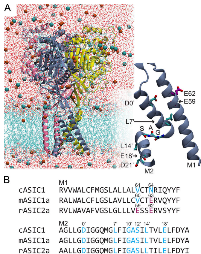
Figure 1. ASIC membrane-spanning region. (A) Left, MD simulation system for rASIC2a model based on PDB accession no. 4NTW (each subunit a different color) embedded in a lipid bilayer (cyan) in NaCl solution (water, red and white sticks; Na + and Cl - , orange and cyan balls). Right, magnified view of M1 and M2 from a single subunit, showing residues discussed in main text. Residues G10', A11', S12', shown in single letter code. (B) M1 and M2 segments from an amino acid sequence alignment of chick ASIC1 (cASIC1), mouse ASIC1a (mASIC1a), and rat ASIC2a (rASIC2a). (The chick ASIC1 gene does not undergo splicing like mammalian ASIC1, hence the single cASIC1 product.) mASIC1a amino acid sequence is 89% and 98% identical to cASIC1 and human ASIC1a, respectively. rASIC2a is 64% and 99% identical to cASIC1 and human ASIC2a, respectively.
