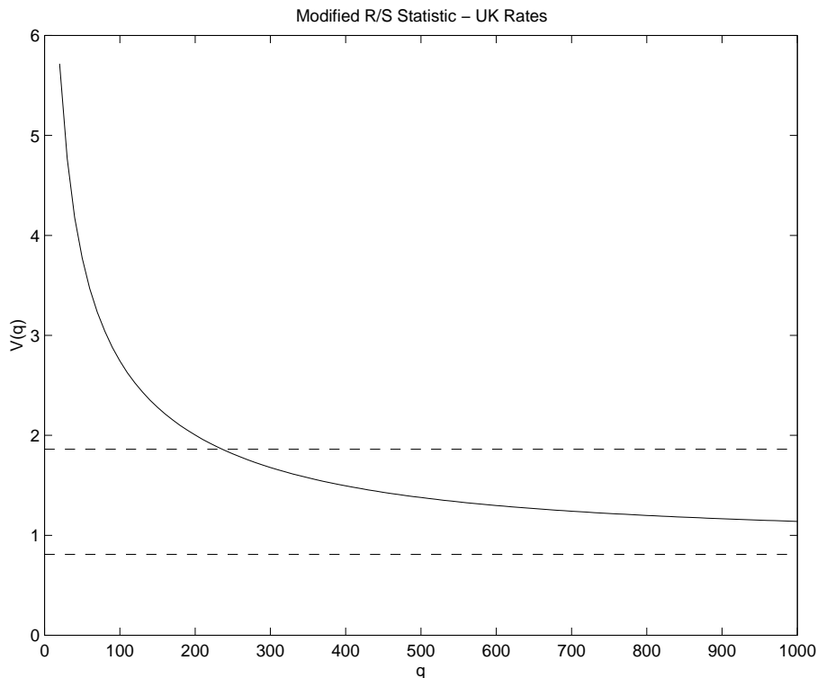
Figure 8: Lo's modified R/S statistic for UK interest rates
