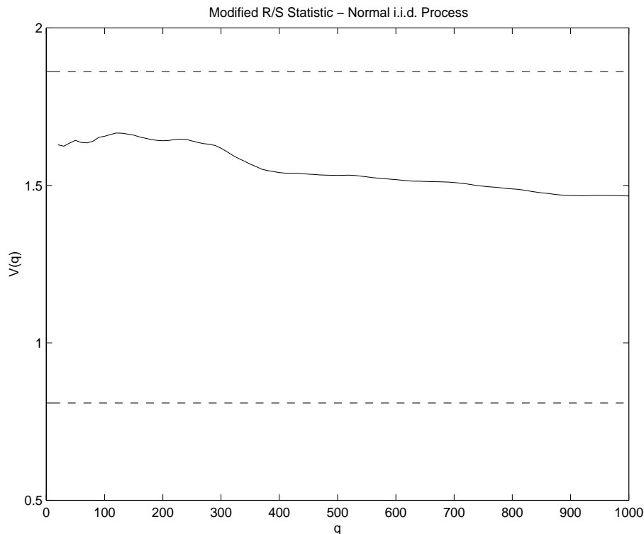
Figure 9: Lo's modified R/S statistic for normal i.i.d. process
