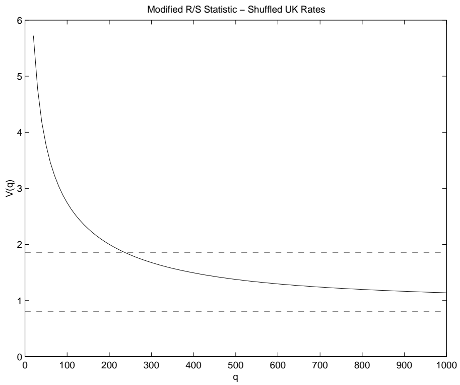
Figure 16: Lo's modified R/S statistic for shuffled UK interest rates, with short-range dependence destroyed
