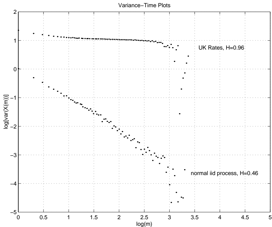
Figure 2: Variance-time plots for UK interest rates and for a normal i.i.d process
