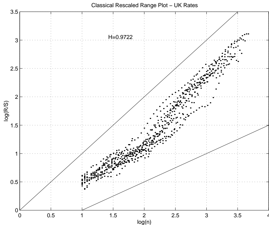
Figure 3: R/S plot for UK interest rates. The straight lines are of slope 0.5 and 1.0 and are included as visual aids.
