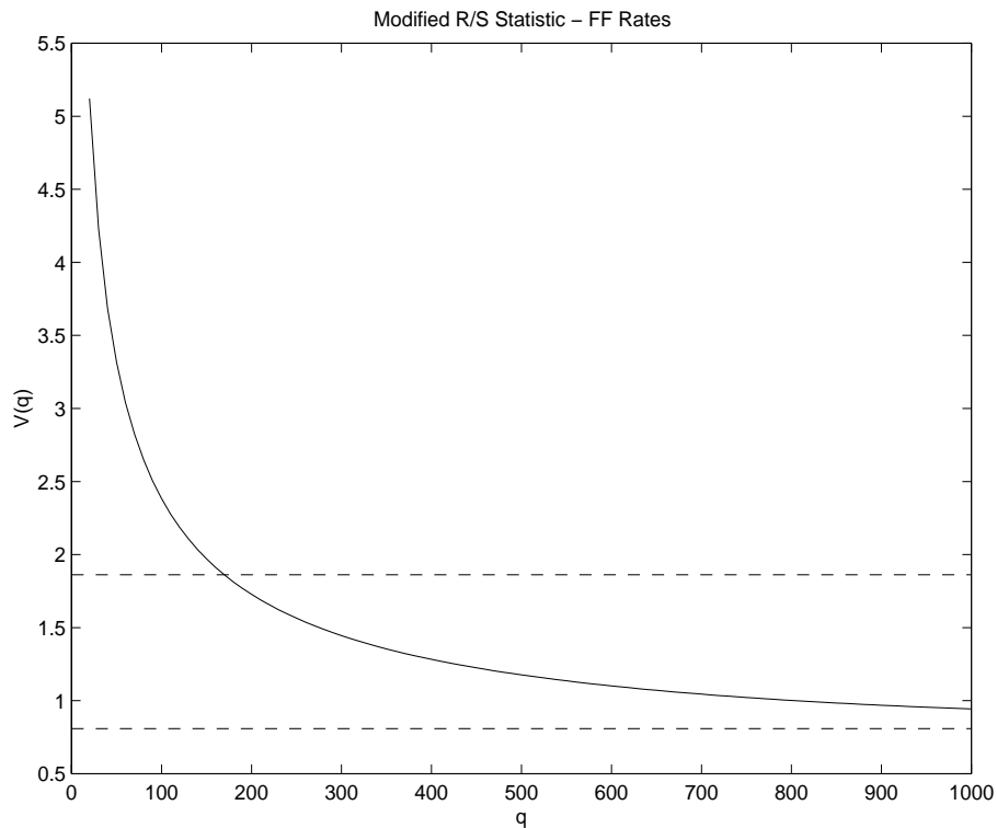
Figure 11: Lo's modified R/S statistic for FF interest rates
