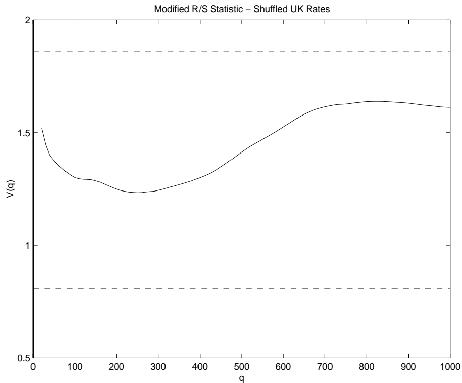
Figure 14: Lo's modified R/S statistic for shuffled UK interest rates, with long-range dependence destroyed
