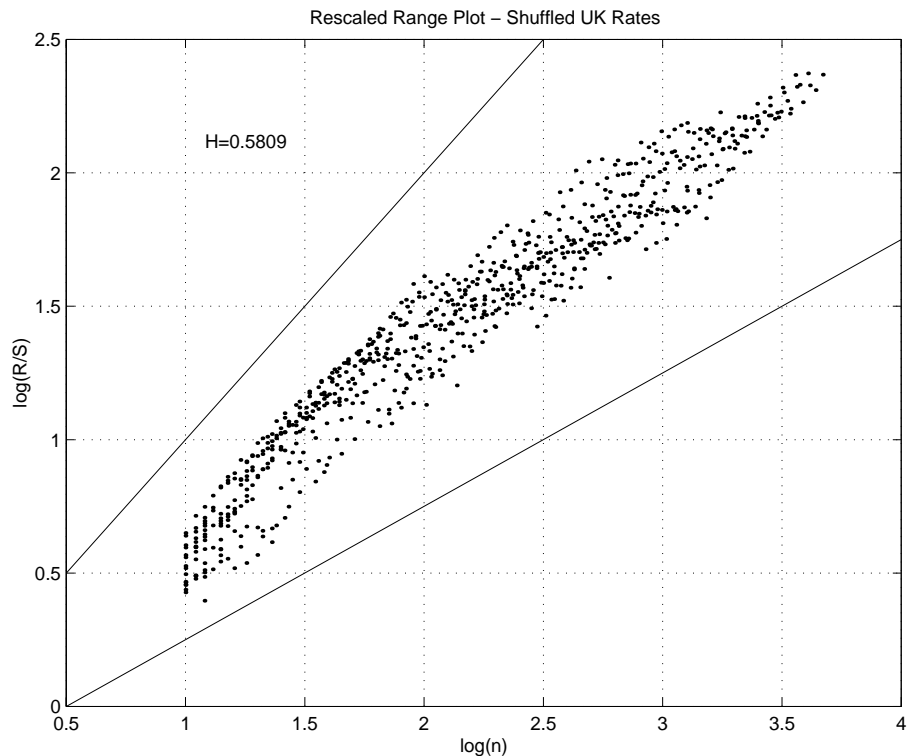
Figure 13: R/S statistic for shuffled UK interest rates, with long-range dependence destroyed
