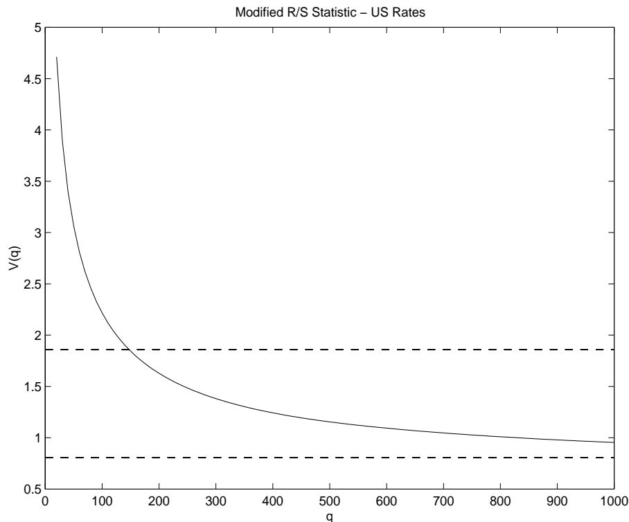
Figure 10: Lo's modified R/S statistic for US interest rates
