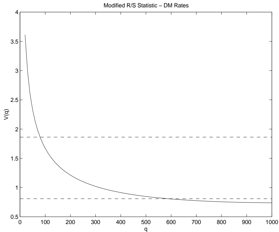
Figure 12: Lo's modified R/S statistic for DM interest rates
