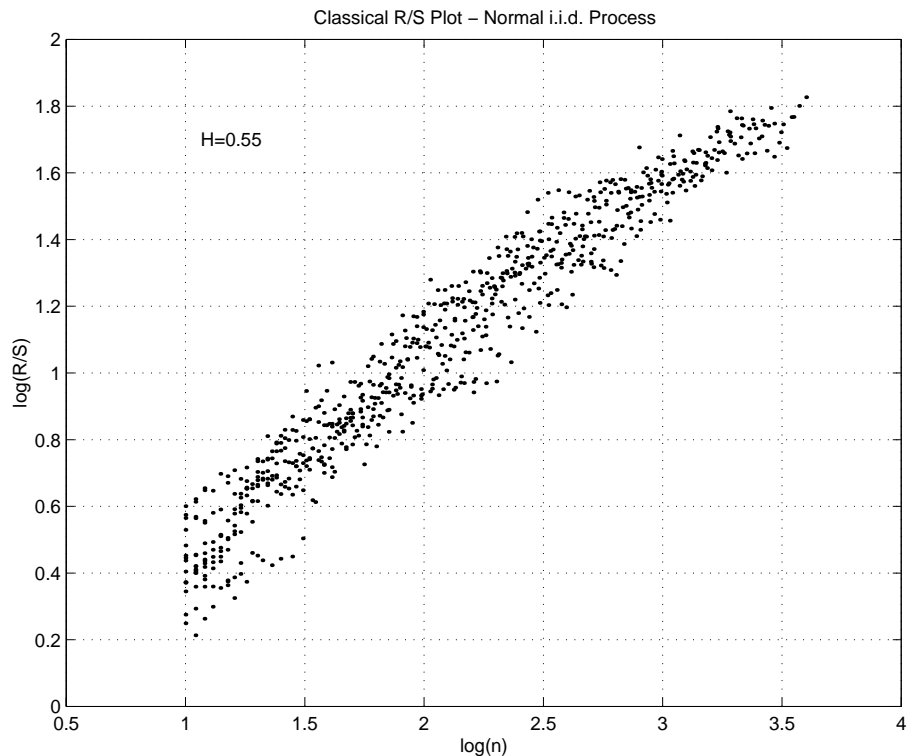
Figure 4: R/S plot for normal i.i.d. process
