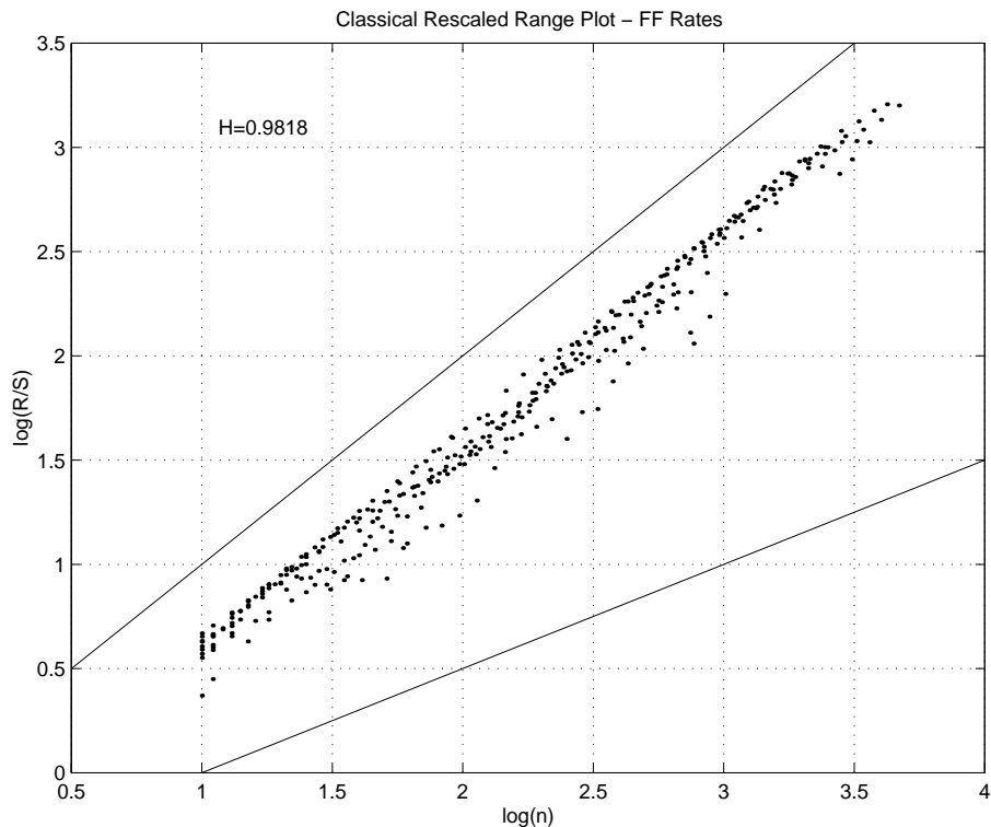
Figure 6: R/S plot for French Franc interest rates
