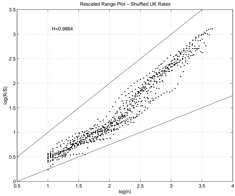
Figure 15: R/S statistic for shuffled UK interest rates, with short-range dependence destroyed
