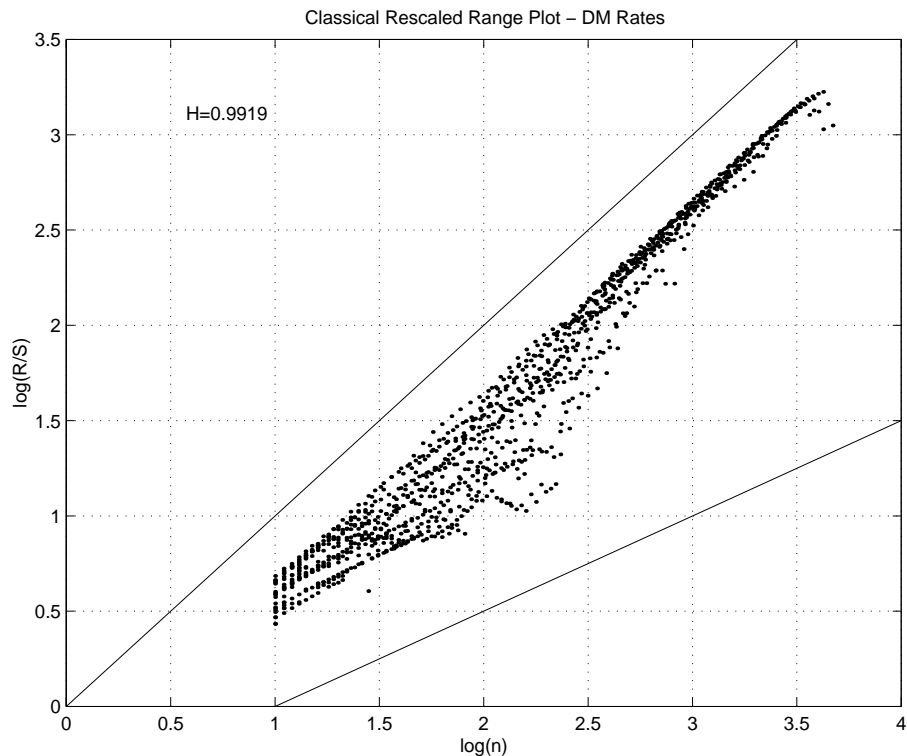
Figure 7: R/S plot for DM interest rates
