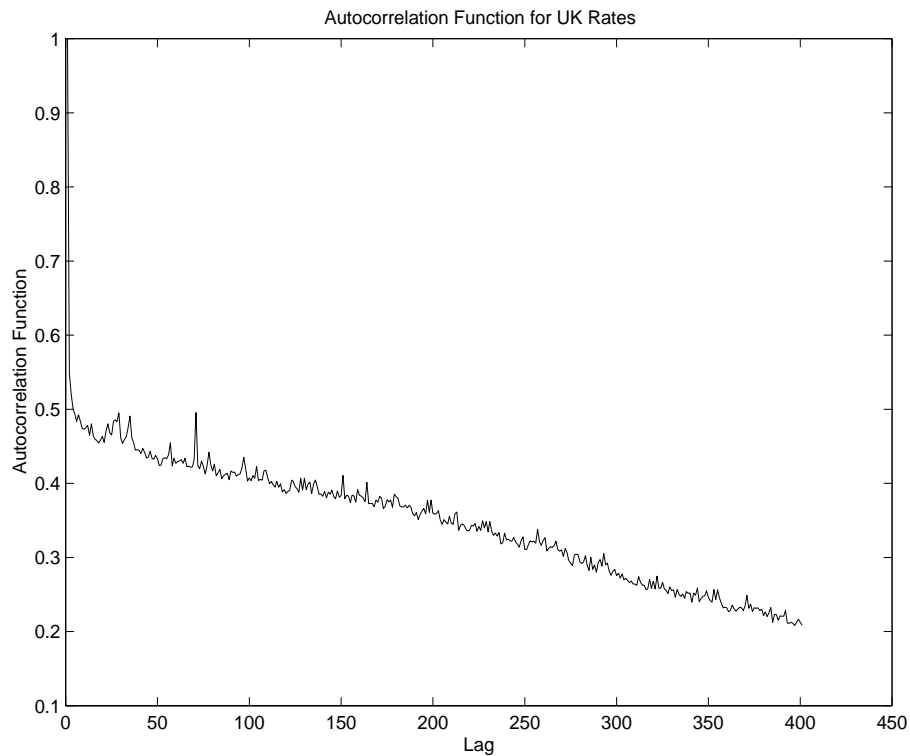
Figure 1: Autocorrelation function for UK interest rates
