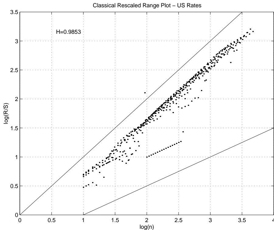
Figure 5: R/S plot for US interest rates
