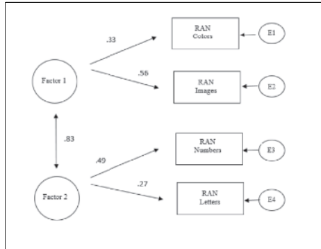
Figure 2. Path diagram of the CFA model in 5 years old children
