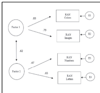
Figure 1. Path diagram of the CFA model in 4 years old children
