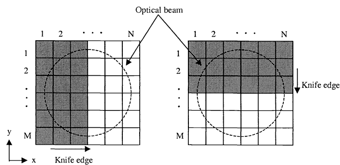
Fig.3 (a) Method to create a moving knife-edge on the DMD TM , (b) 3-dimensional beam profile constructed from 2-dimensional knife edge measurement data. Pixel Pitch: 13.8 micron. Laser Beam Wavelength: 1550 nm.
