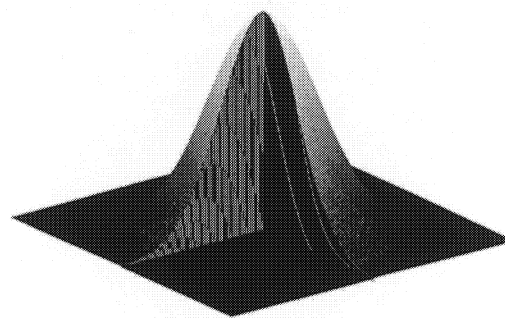
Fig.3 (a) Method to create a moving knife-edge on the DMD TM , (b) 3-dimensional beam profile constructed from 2-dimensional knife edge measurement data. Pixel Pitch: 13.8 micron. Laser Beam Wavelength: 1550 nm.
