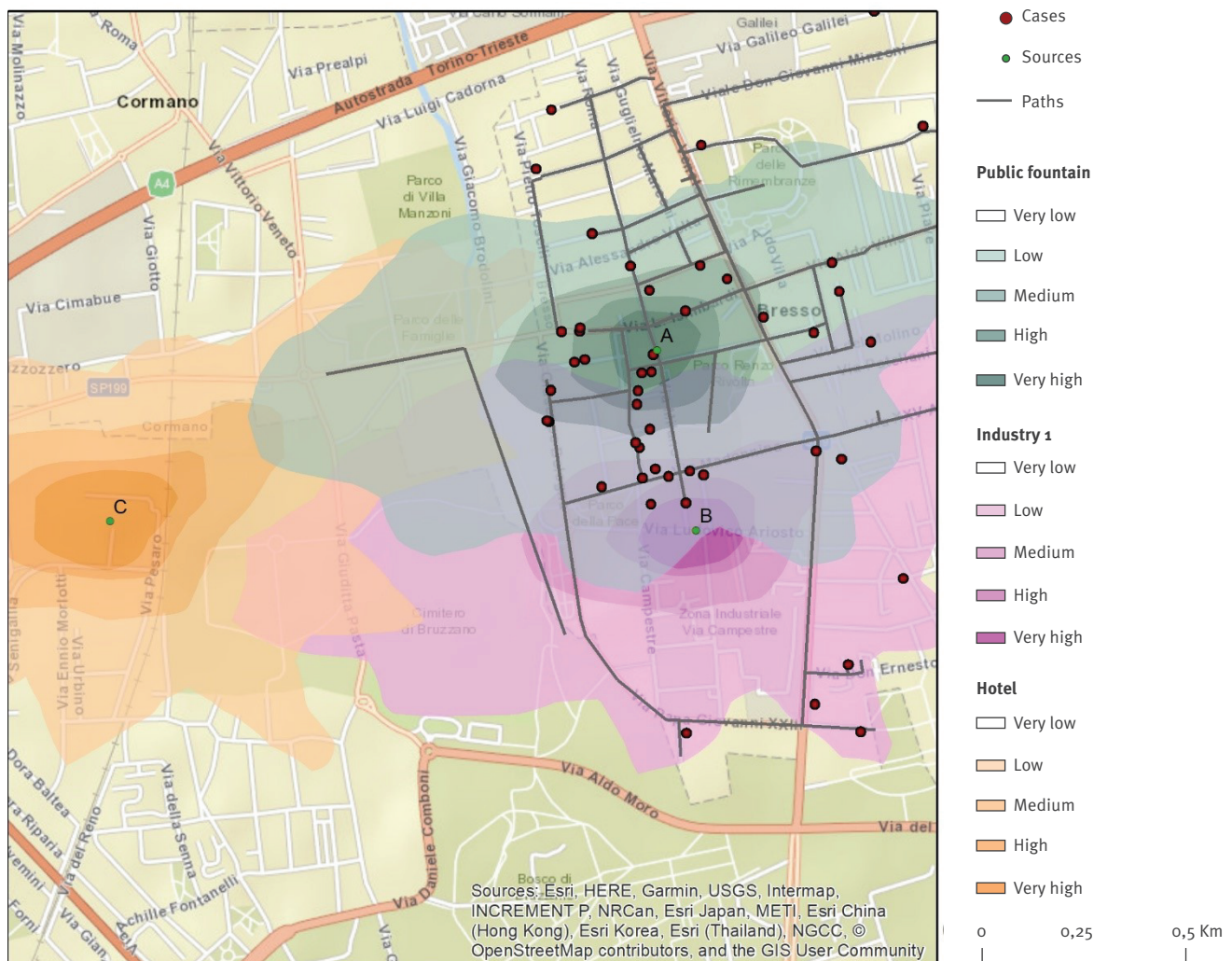
Public fountain (site A), cooling tower of Industry 1 (site B) and hotel (site C). Different colours represent the intensity of concentration within each plume.
