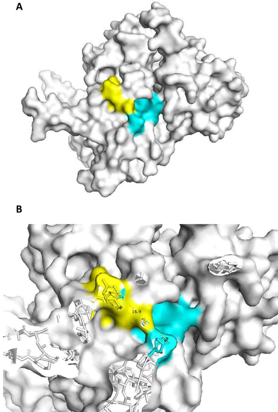
Fig. 2. Epitope mapping into 6M3M structural model. The figure depicts mapping of the epitope sequence AQPAPSASAFFGMSR (yellow) and QFAPSASAFFGMSRIGM (cyan). A-panel shows the surface mapping of the epitopes in the D structure of the nucleocapsid protein domain. B-panel highlights distances occurring between the mapped epitopes.
