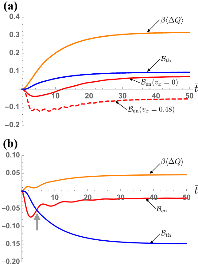
FIG. 1. Time evolution of the bounds \mathcal{B}_{en} and \mathcal{B}_{th} , and the mean dissipated heat ( \Delta Q ) for several initial conditions. (a) We compare their time evolutions for two different initial conditions with the same population without coherence [ \mathbf{v}_1(0) = (0, 0, 0.28) : solid lines] and with coherence [ \mathbf{v}_2(0) = (0.48, 0, 0.28) : dashed lines]. Solid lines and dashed lines coincide for the mean dissipated heat (orange line) and the thermodynamic bound (blue line), whereas they diverge for the entropic bound (red lines). (b) We plot their time evolutions for another initial state different from the solid lines in (a) in their initial populations [ \mathbf{v}_3(0) = (0, 0, -0.5) ]. The gray arrow in the panel indicates crossover of \mathcal{B}_{en} and \mathcal{B}_{th} . Their time evolutions differ from the solid lines in (a), thus the three quantities explicitly depend on the initial populations. In the numerical calculations, we set the parameters to \lambda = 0.1 , \Omega = 0.4 , and \beta = 1 .
