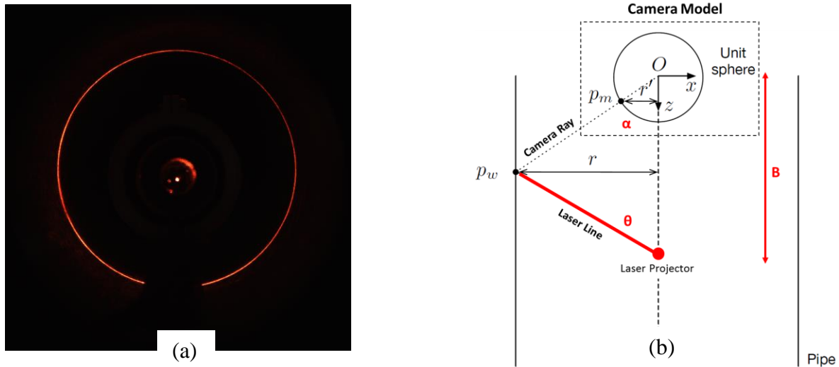
Figure 2 - Laser Profiler Image (a) Laser Image (b) Camera Laser Geometry
