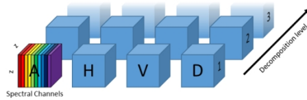
Figure 1. The methodological framework, the spectral dimension is colored after every step for the sake of a better and easier visualization. (1.1) a generic hyperspectral data cube; (1.2) the data structure obtained after the 2D-SWT decomposition; (1.3) GLCM obtained from each slab of the wavelet coefficient three-dimensional arrays depicted in 1.2; (1.4) the descriptors calculated from the GLCM; (1.5) rearrangement of the descriptors matrix.
